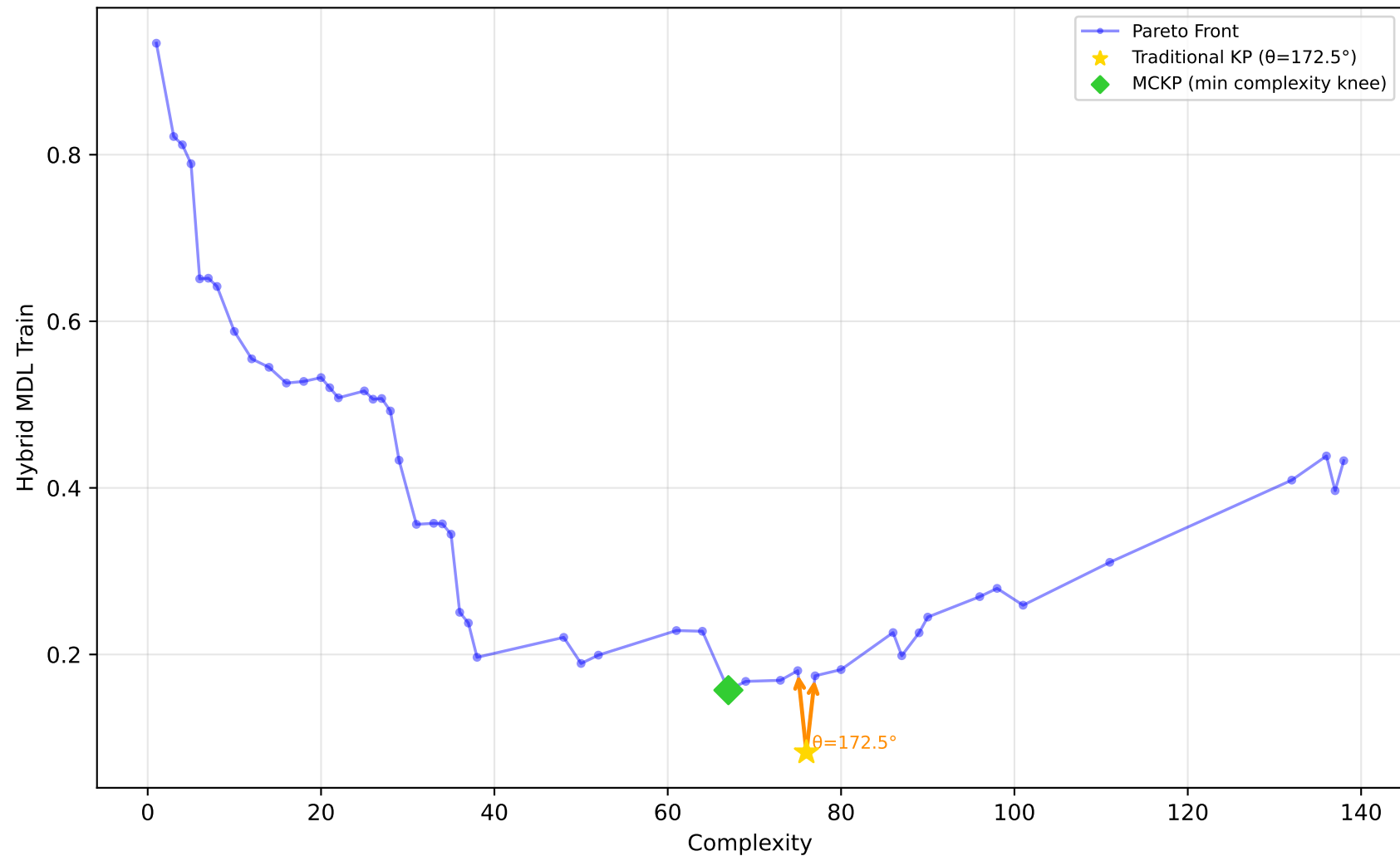
589_fri_c2_1000_25 - Run 2 - MVP - Hybrid MDL Train \lambda_1=0.00, \bar{\lambda}_2=0.00, \bar{\lambda}_3=0.00 | Difficulty: 1.00 | Method: hmr
