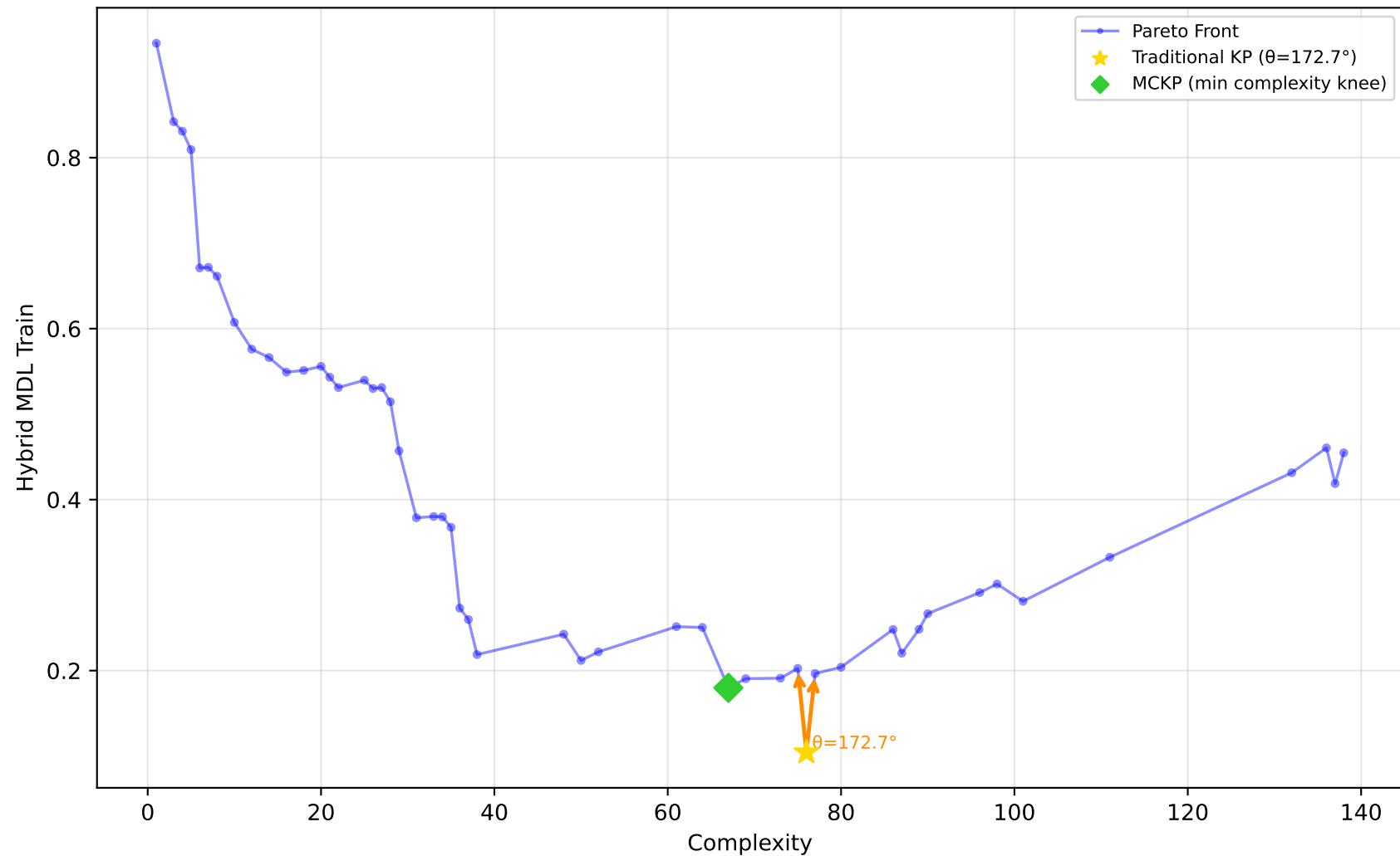
589_fri_c2_1000_25 - Run 2 - MVP - Hybrid MDL Train \lambda_1=0.30, \bar{\lambda}_2=0.00, \bar{\lambda}_3=0.20 | Difficulty: 1.00 | Method: hmr
