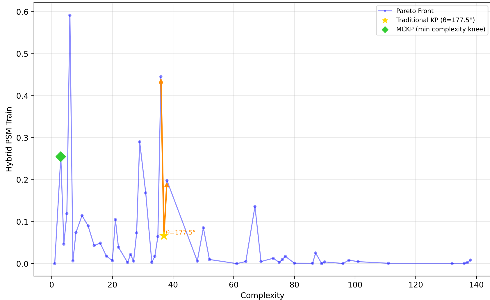
589_fri_c2_1000_25 - Run 2 - MVP - Hybrid PSM Train \lambda_1=0.00, \bar{\lambda}_2=0.00, \bar{\lambda}_3=0.00 | Difficulty: 1.00 | Method: hmr
