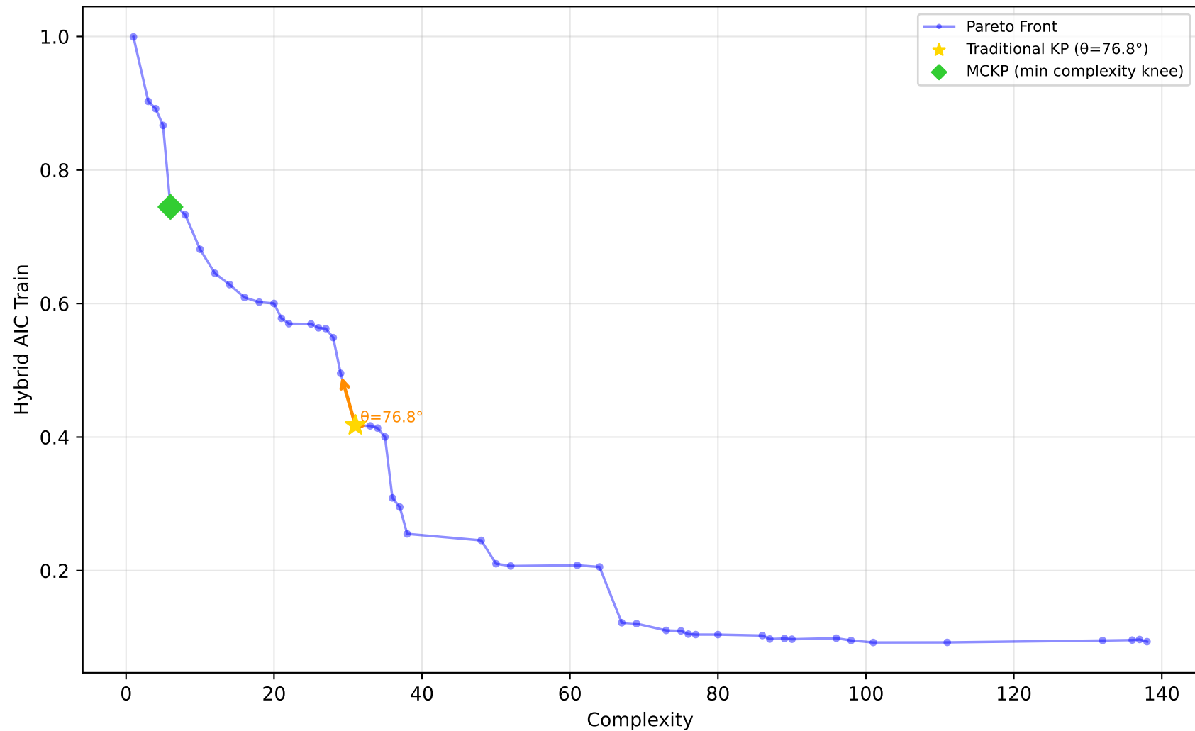
589_fri_c2_1000_25 - Run 2 - SVP - Hybrid AIC Train \lambda_1=0.10, \lambda_2=0.00, \lambda_3=0.10 | Difficulty: 1.00 | Method: hmr
