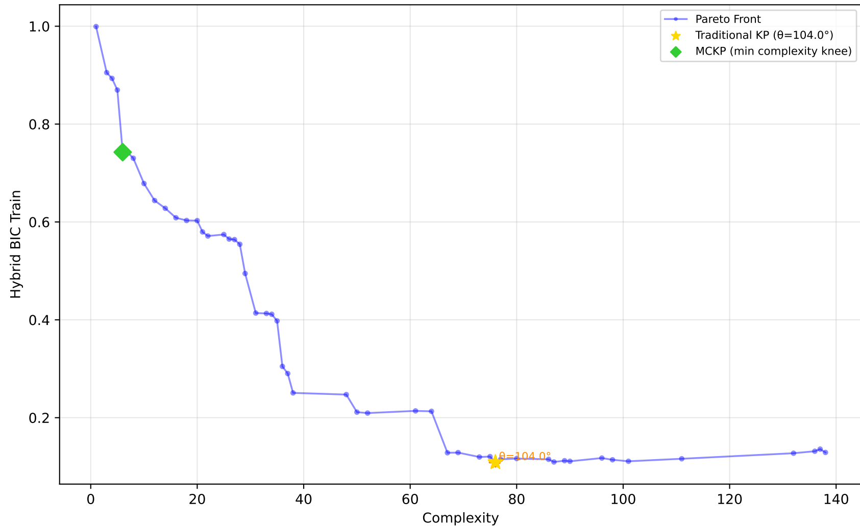
589_fri_c2_1000_25 - Run 2 - SVP - Hybrid BIC Train \lambda_1=0.20 , \lambda_2=0.00 , \lambda_3=1.00 | Difficulty: 1.00 | Method: hmr
