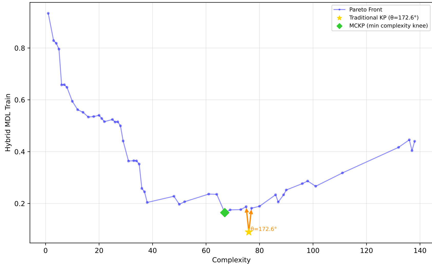
589_fri_c2_1000_25 - Run 2 - SVP - Hybrid MDL Train \lambda_1=0.10, \bar{\lambda}_2=0.00, \bar{\lambda}_3=0.10 | Difficulty: 1.00 | Method: hmr
