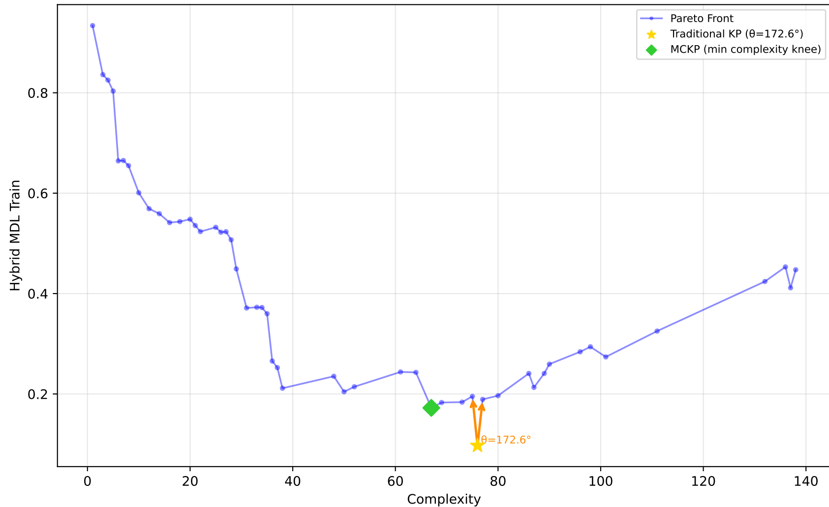
589_fri_c2_1000_25 - Run 2 - SVP - Hybrid MDL Train \lambda_1=0.20, \lambda_2=0.00, \lambda_3=1.00 | Difficulty: 1.00 | Method: hmr
