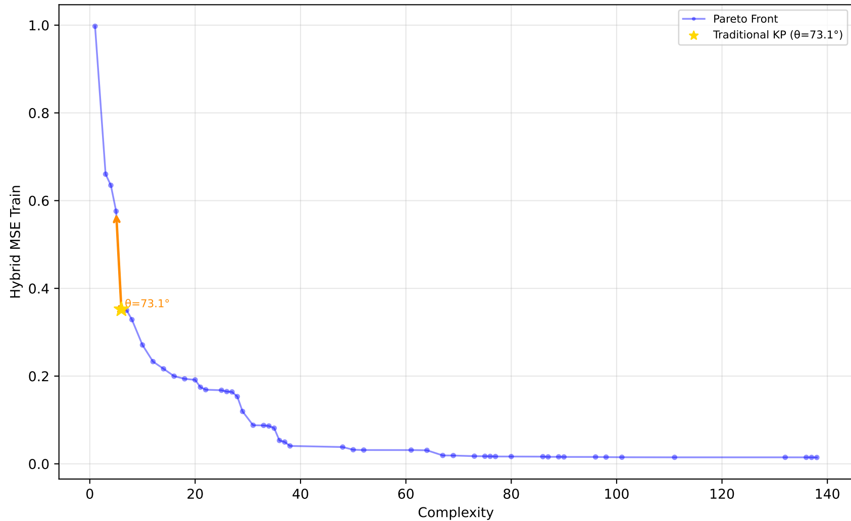
589_fri_c2_1000_25 - Run 2 - SVP - Hybrid MSE Train \lambda_1=0.10, \lambda_2=0.00, \lambda_3=0.10 | Difficulty: 1.00 | Method: hmr
