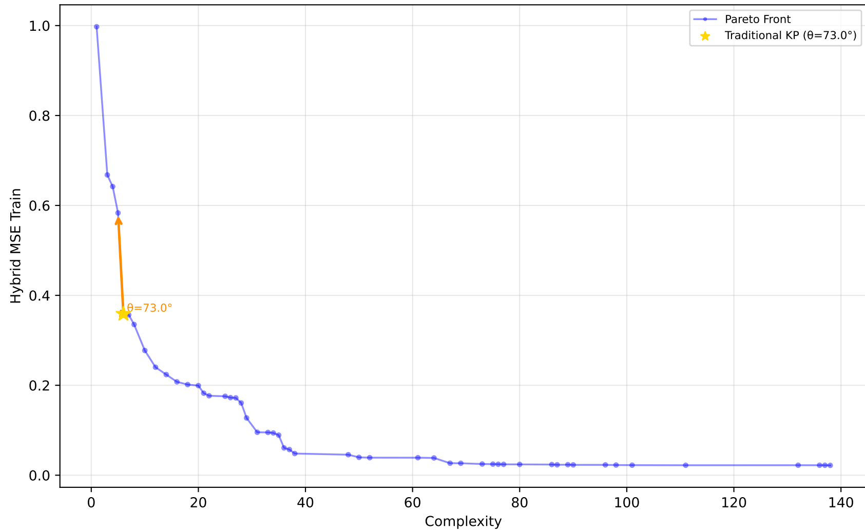
589_fri_c2_1000_25 - Run 2 - SVP - Hybrid MSE Train \lambda_1=0.20 , \lambda_2=0.00 , \lambda_3=1.00 | Difficulty: 1.00 | Method: hmr
