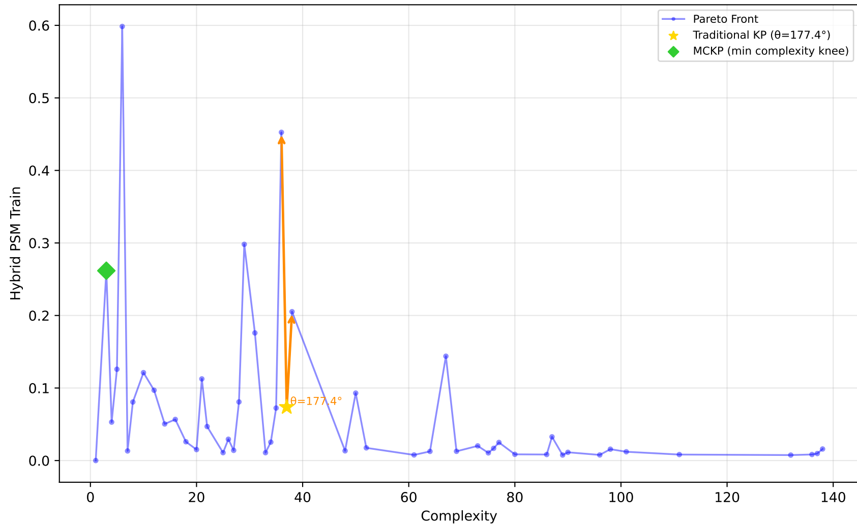
589_fri_c2_1000_25 - Run 2 - SVP - Hybrid PSM Train \lambda_1=0.10, \lambda_2=0.00, \lambda_3=0.10 | Difficulty: 1.00 | Method: hmr
