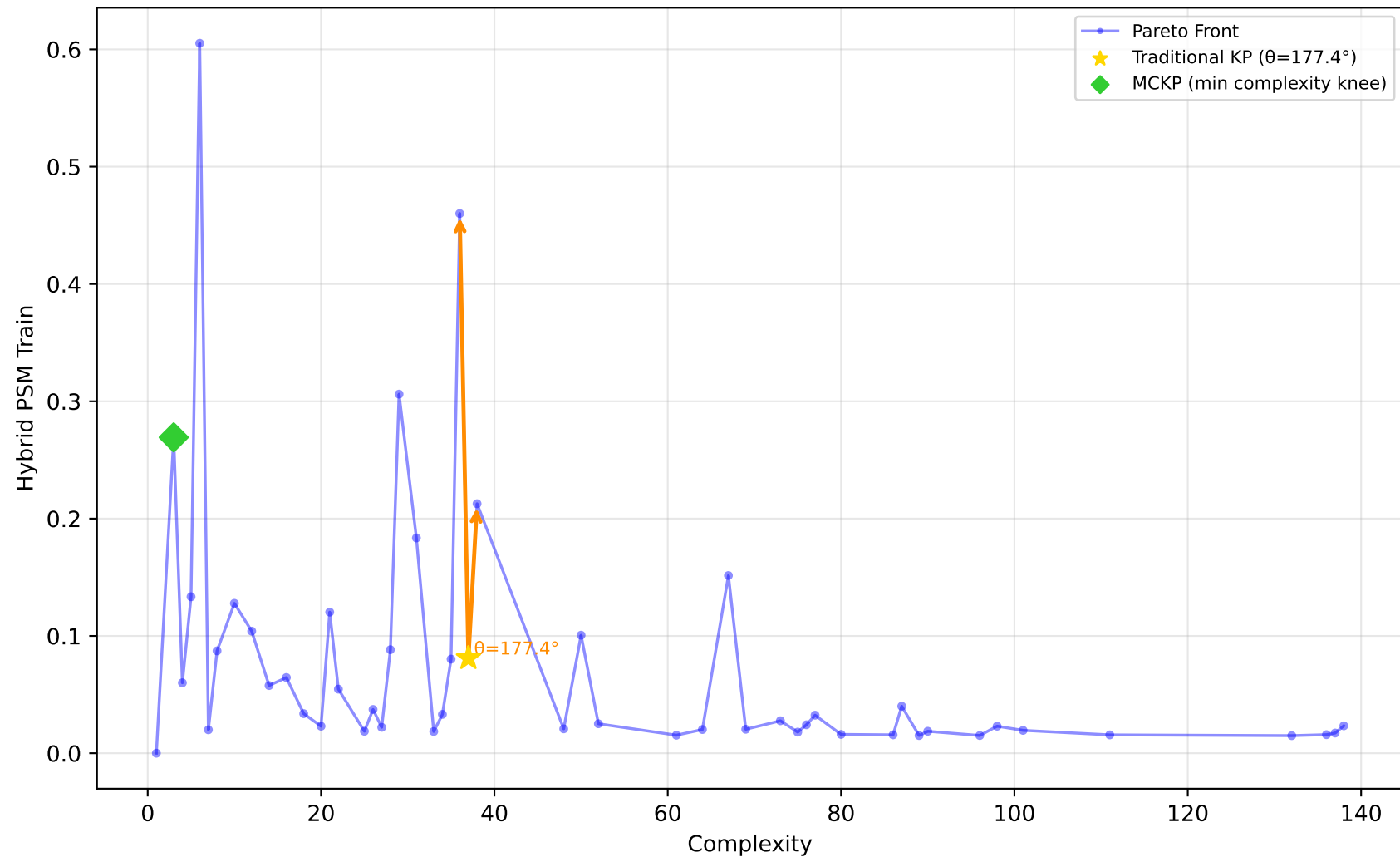
589_fri_c2_1000_25 - Run 2 - SVP - Hybrid PSM Train \lambda_1=0.20, \lambda_2=0.00, \lambda_3=1.00 | Difficulty: 1.00 | Method: hmr
