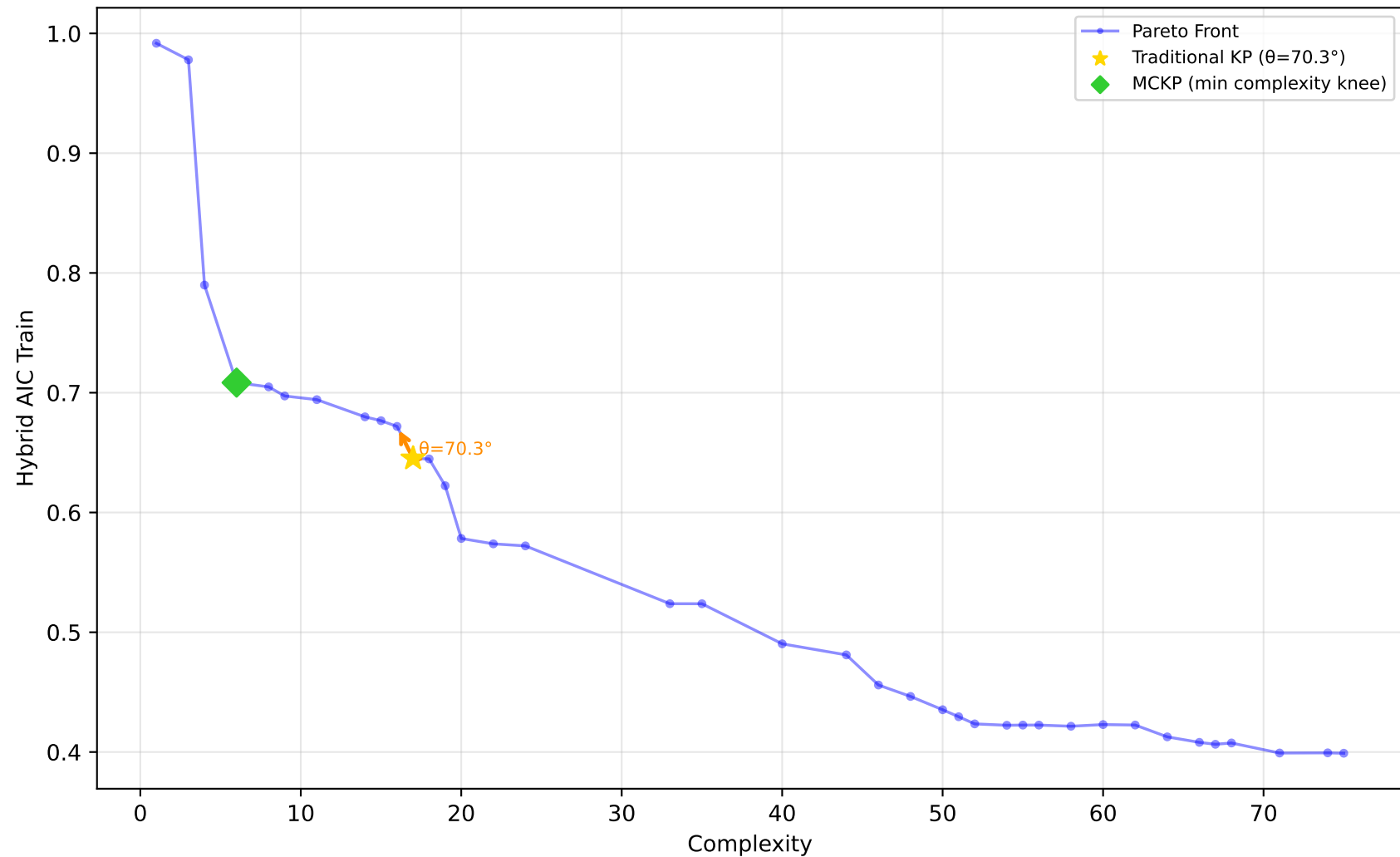
589_fri_c2_1000_25 - Run 30 - MVP - Hybrid AIC Train \lambda_1=0.00, \lambda_2=0.00, \lambda_3=0.00 | Difficulty: 1.00 | Method: hmr
