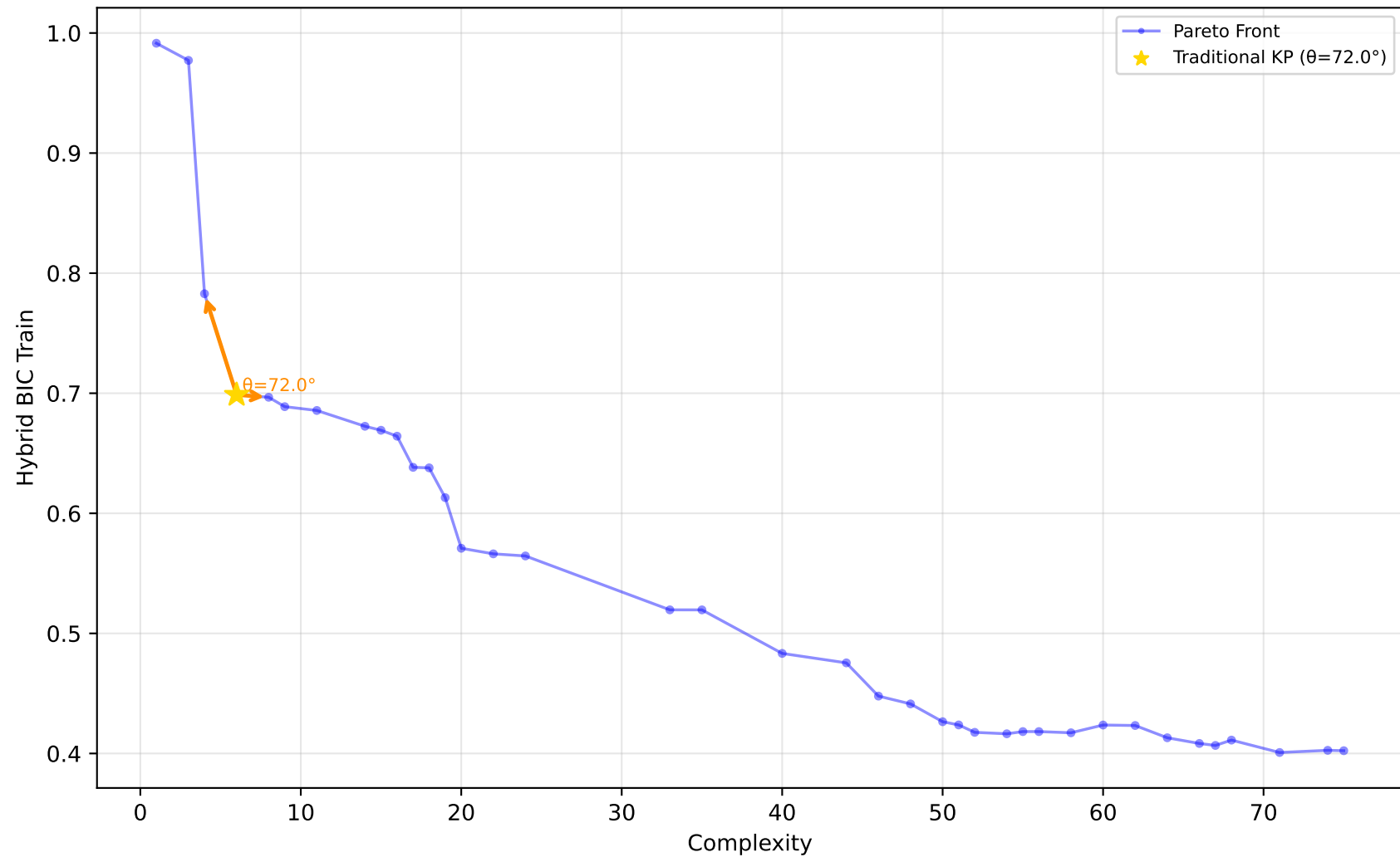
589_fri_c2_1000_25 - Run 30 - MVP - Hybrid BIC Train \lambda_1=0.00, \bar{\lambda}_2=0.00, \bar{\lambda}_3=0.00 | Difficulty: 1.00 | Method: hmr
