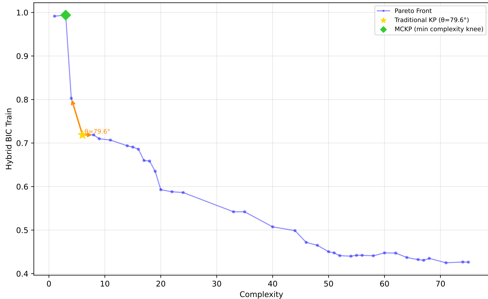
589_fri_c2_1000_25 - Run 30 - MVP - Hybrid BIC Train \lambda_1=0.30, \bar{\lambda}_2=0.00, \bar{\lambda}_3=0.20 | Difficulty: 1.00 | Method: hmr
