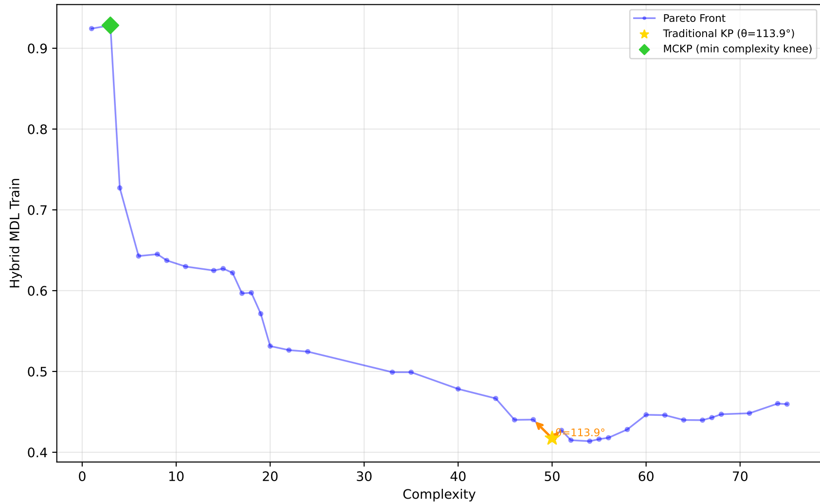
589_fri_c2_1000_25 - Run 30 - MVP - Hybrid MDL Train \lambda_1=0.30, \lambda_2=0.00, \lambda_3=0.20 | Difficulty: 1.00 | Method: hmr
