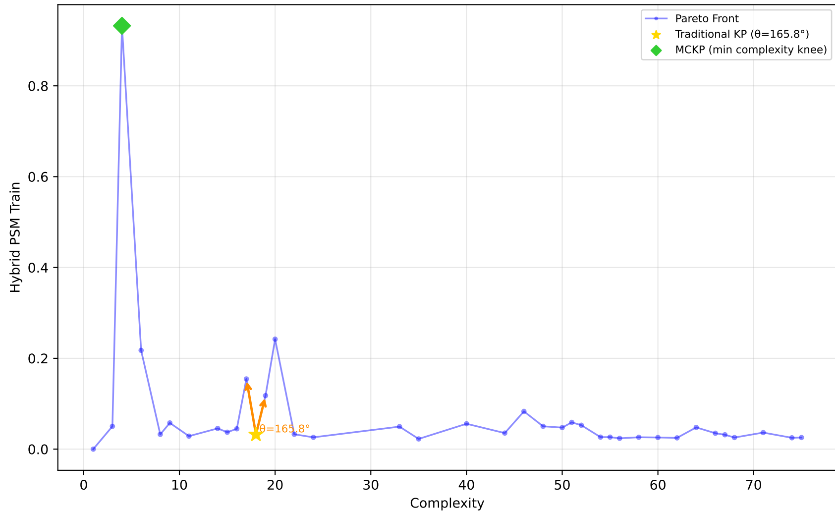
589_fri_c2_1000_25 - Run 30 - MVP - Hybrid PSM Train \lambda_1=0.30, \lambda_2=0.00, \lambda_3=0.20 | Difficulty: 1.00 | Method: hmr
