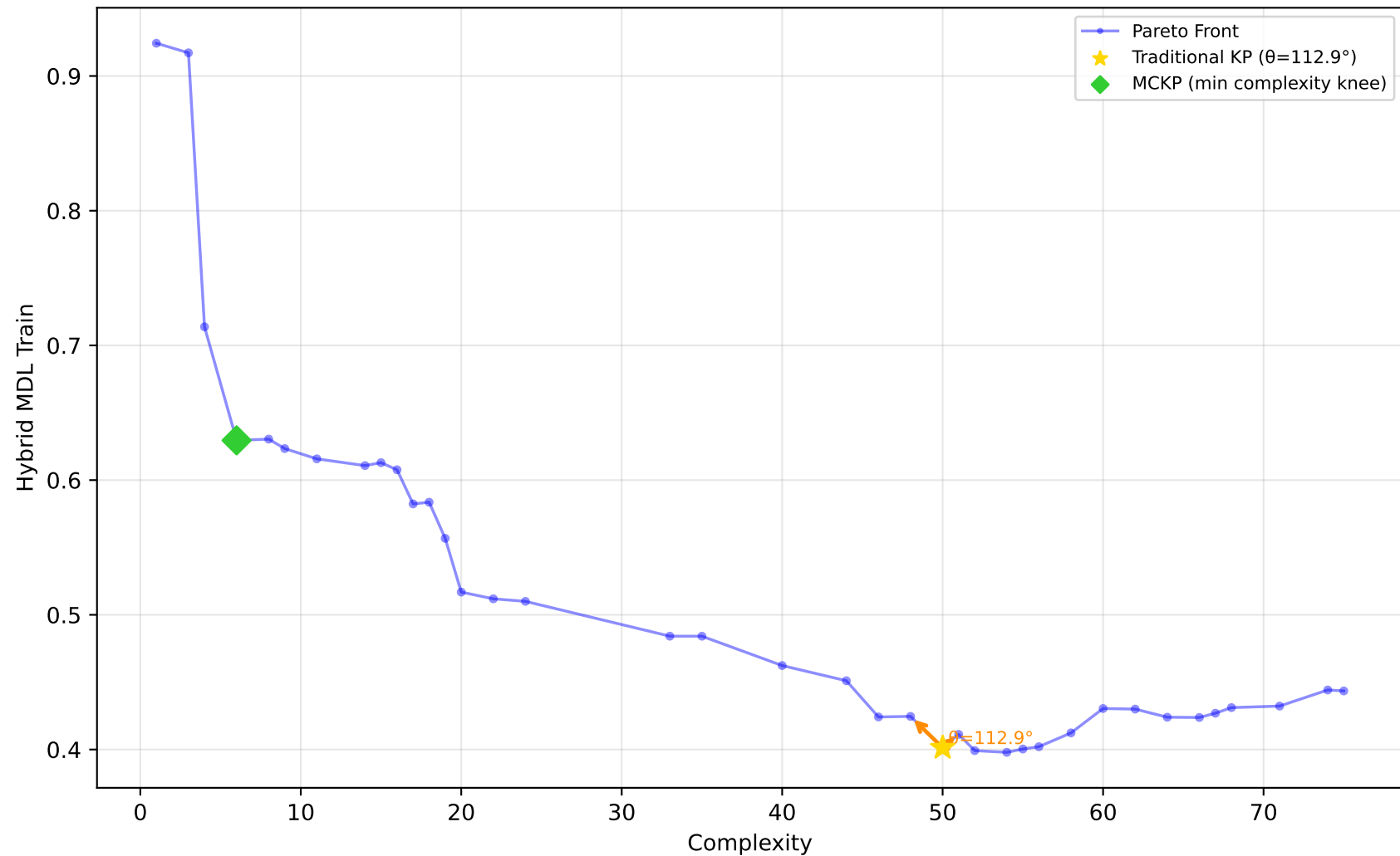
589_fri_c2_1000_25 - Run 30 - SVP - Hybrid MDL Train \lambda_1=0.10, \lambda_2=0.00, \lambda_3=0.10 | Difficulty: 1.00 | Method: hmr
