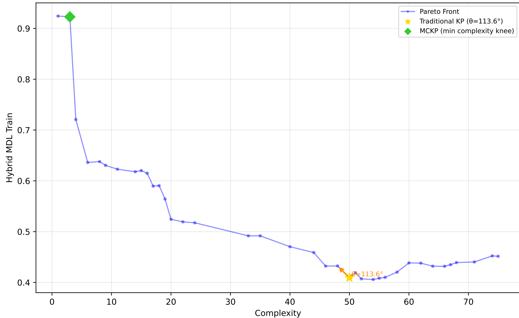
589_fri_c2_1000_25 - Run 30 - SVP - Hybrid MDL Train \lambda_1=0.20, \lambda_2=0.00, \lambda_3=1.00 | Difficulty: 1.00 | Method: hmr
