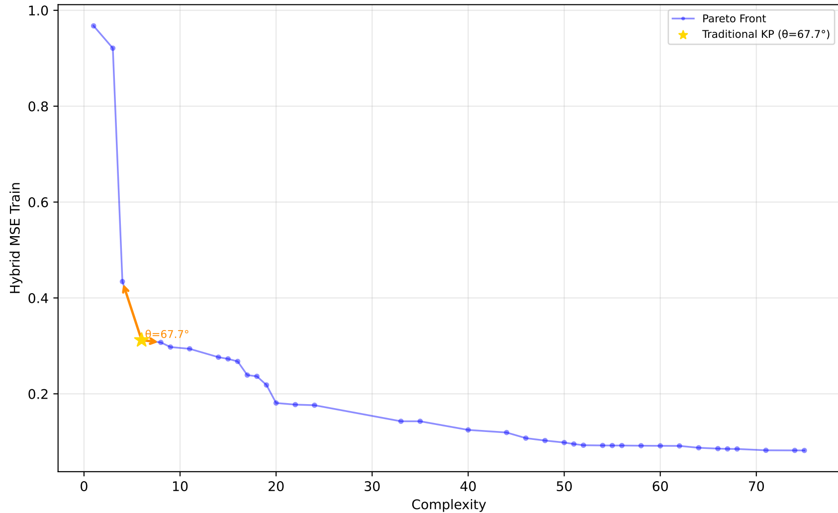
589_fri_c2_1000_25 - Run 30 - SVP - Hybrid MSE Train \lambda_1=0.10, \lambda_2=0.00, \lambda_3=0.10 | Difficulty: 1.00 | Method: hmr
