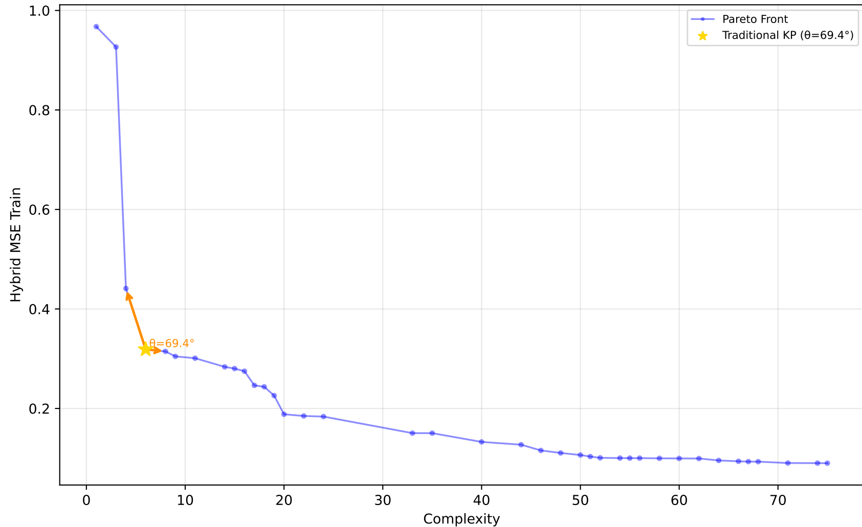
589_fri_c2_1000_25 - Run 30 - SVP - Hybrid MSE Train \lambda_1=0.20, \bar{\lambda}_2=0.00, \bar{\lambda}_3=1.00 | Difficulty: 1.00 | Method: hmr
