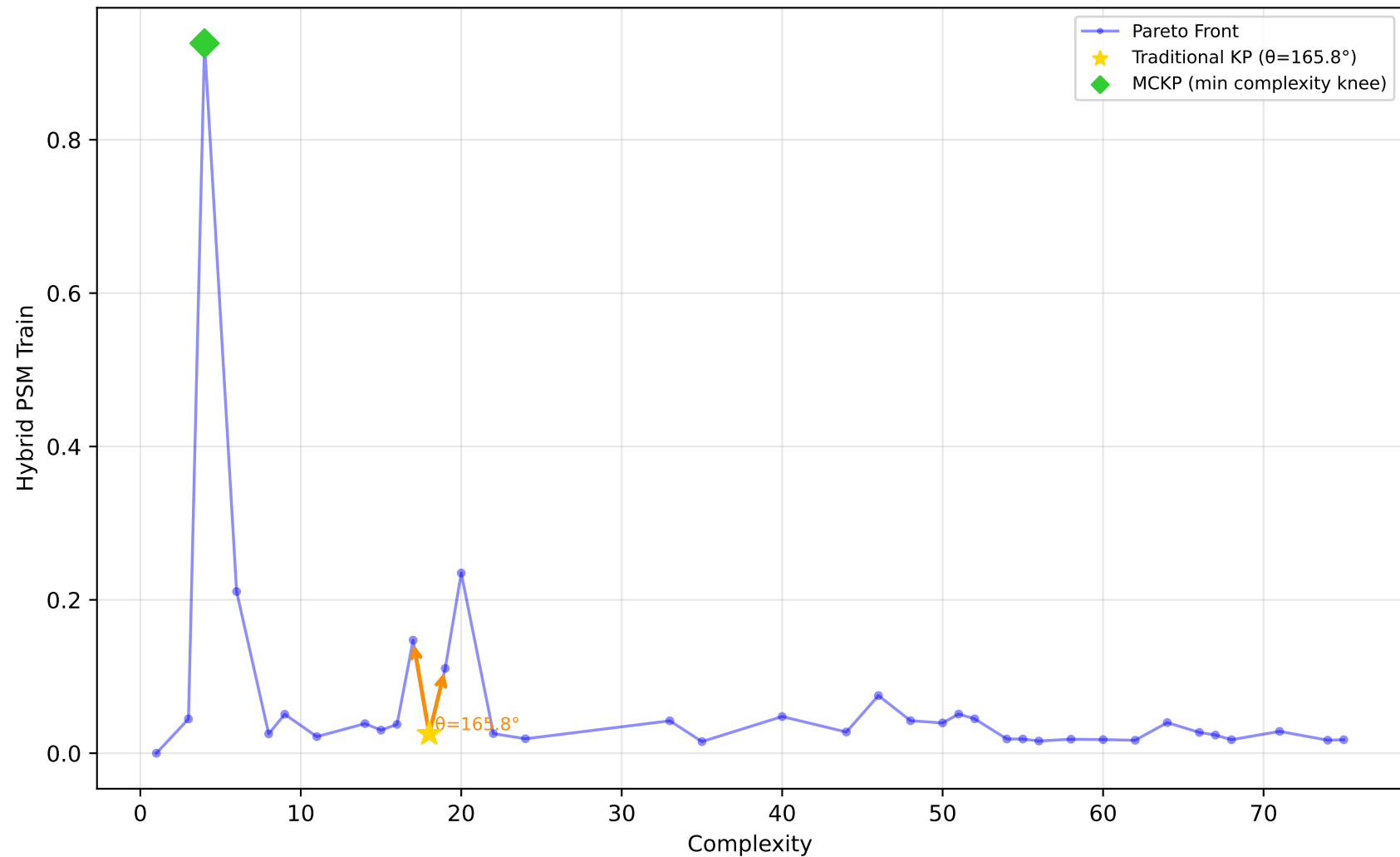
589_fri_c2_1000_25 - Run 30 - SVP - Hybrid PSM Train \lambda_1=0.20, \bar{\lambda}_2=0.00, \bar{\lambda}_3=1.00 | Difficulty: 1.00 | Method: hmr
