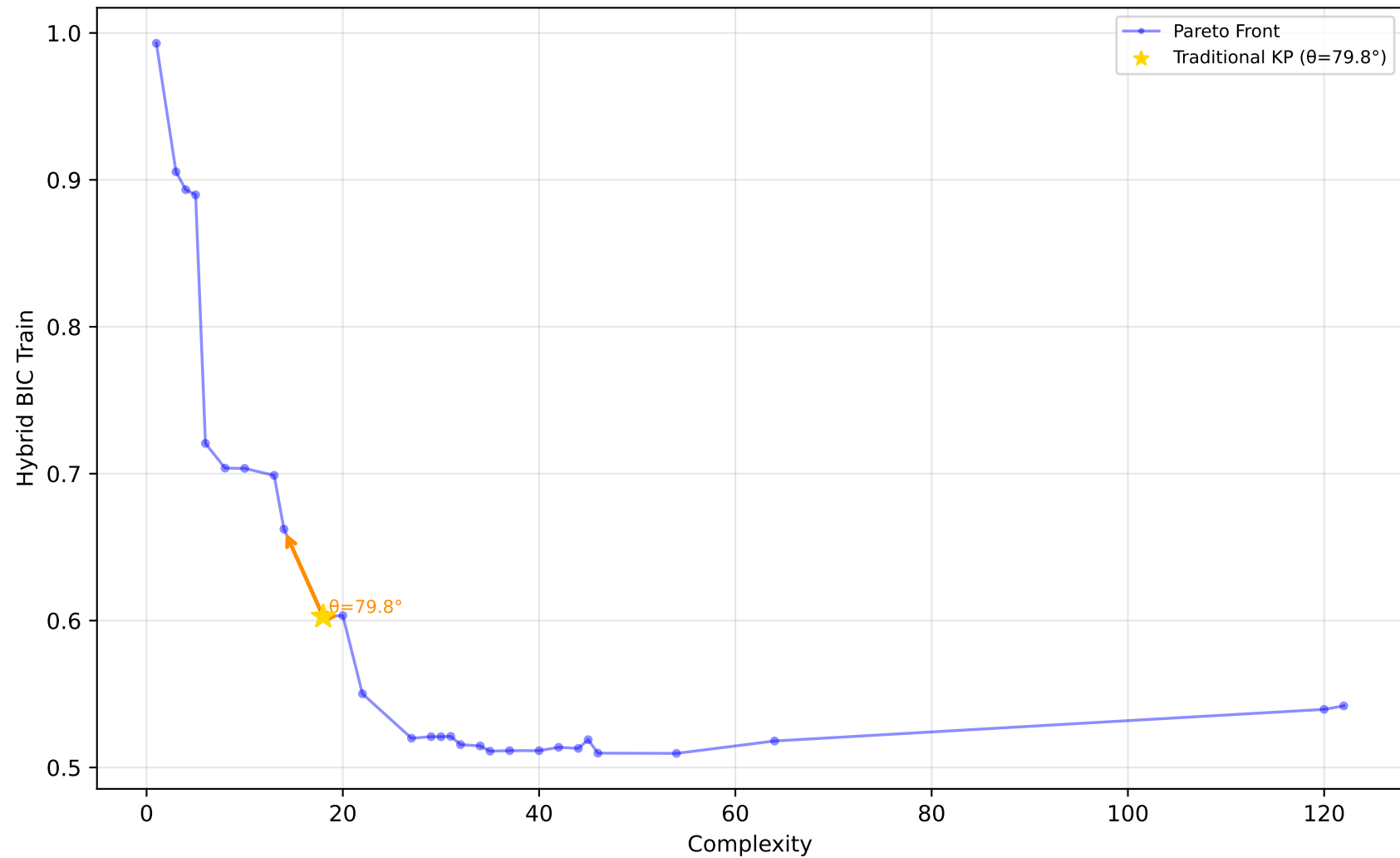
589_fri_c2_1000_25 - Run 3 - MVP - Hybrid BIC Train \lambda_1=0.30 , \lambda_2=0.00 , \lambda_3=0.20 | Difficulty: 1.00 | Method: hmr
