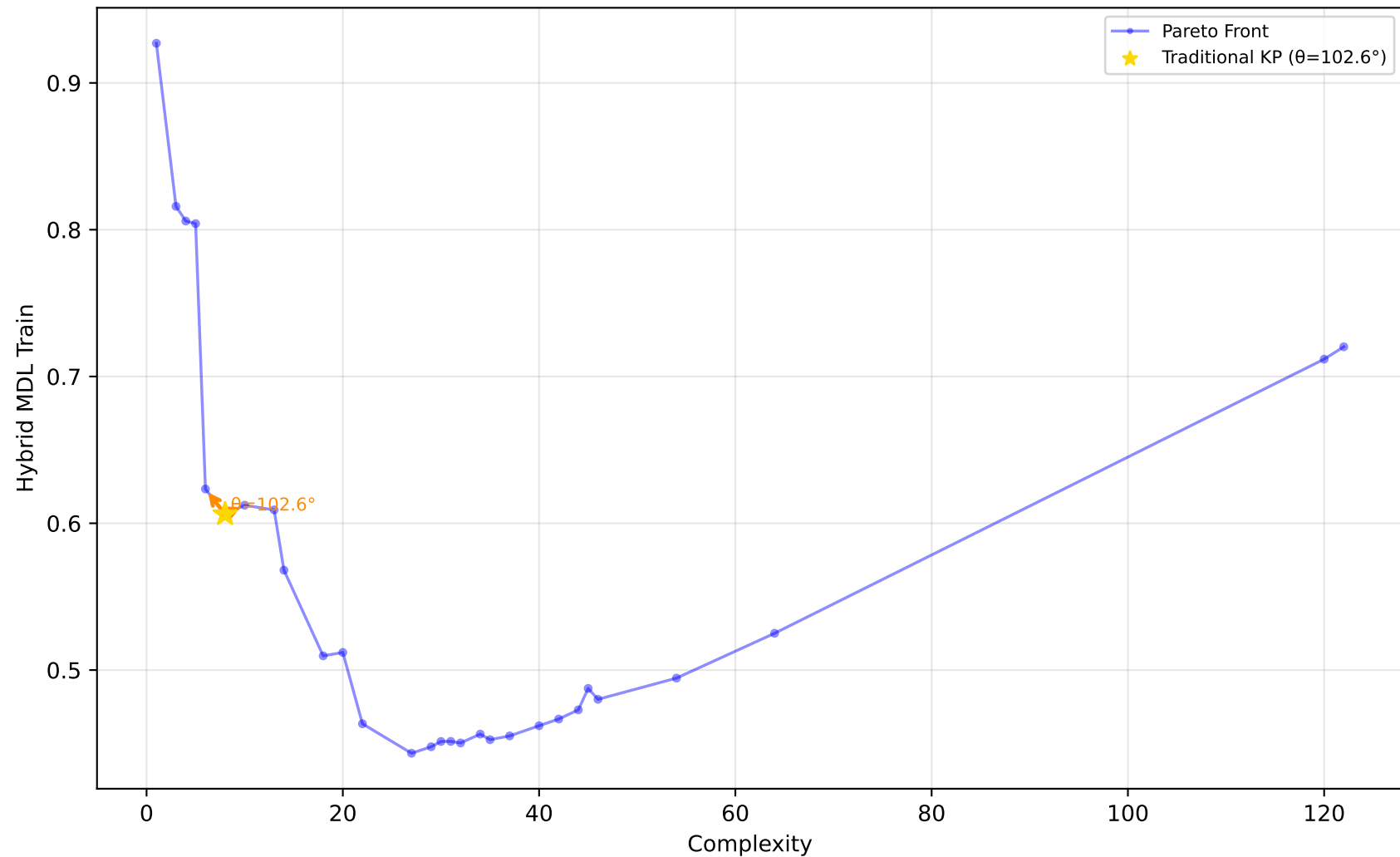
589_fri_c2_1000_25 - Run 3 - MVP - Hybrid MDL Train \lambda_1=0.00, \bar{\lambda}_2=0.00, \bar{\lambda}_3=0.00 | Difficulty: 1.00 | Method: hmr
