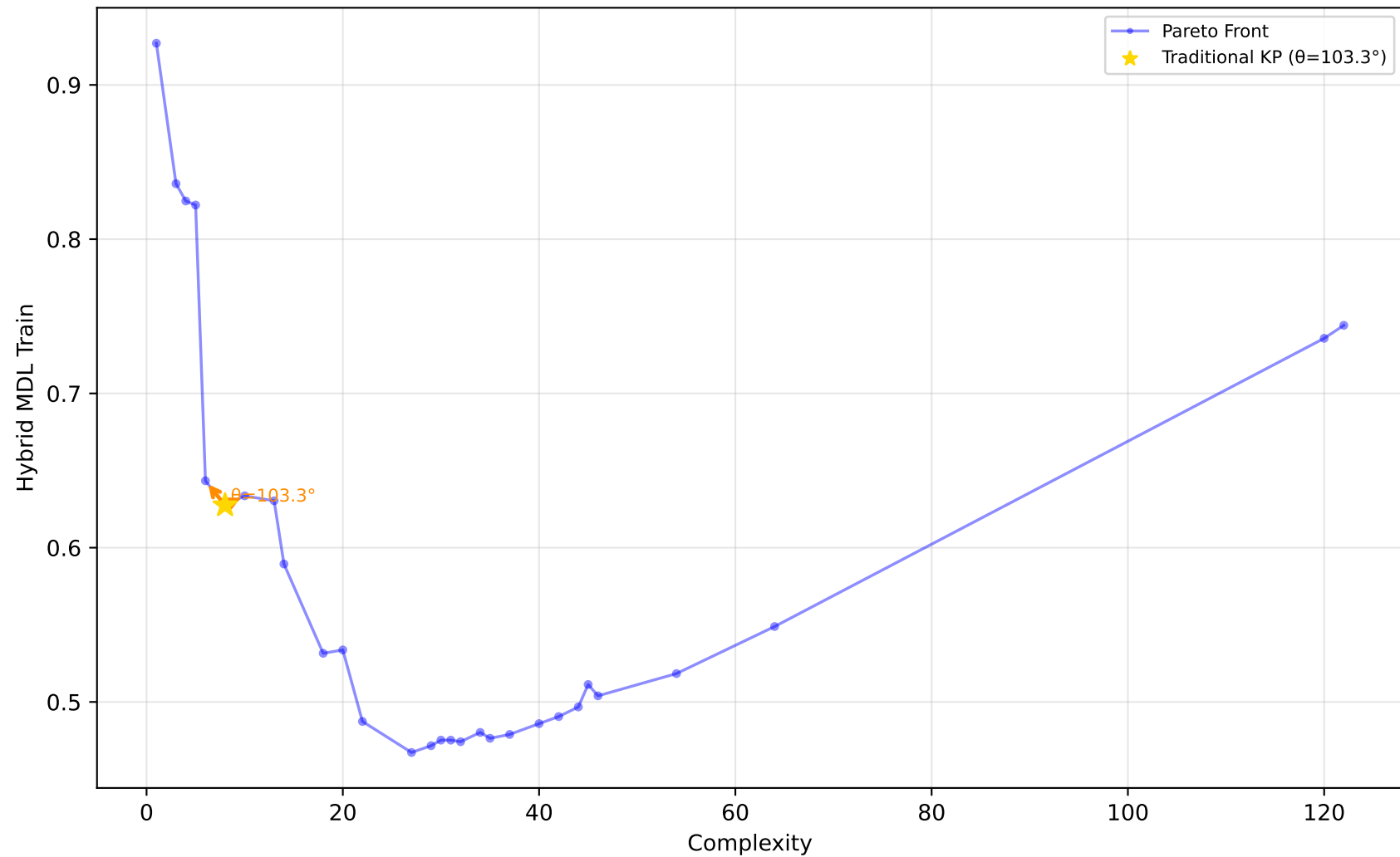
589_fri_c2_1000_25 - Run 3 - MVP - Hybrid MDL Train \lambda_1=0.30, \bar{\lambda}_2=0.00, \bar{\lambda}_3=0.20 | Difficulty: 1.00 | Method: hmr
