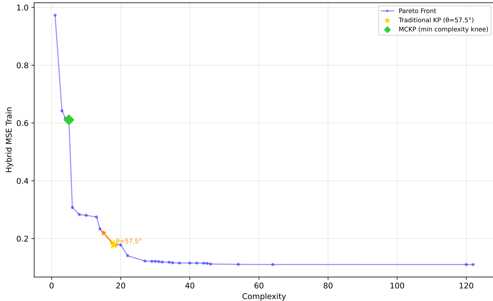
589_fri_c2_1000_25 - Run 3 - MVP - Hybrid MSE Train \lambda_1=0.00, \bar{\lambda}_2=0.00, \bar{\lambda}_3=0.00 | Difficulty: 1.00 | Method: hmr
