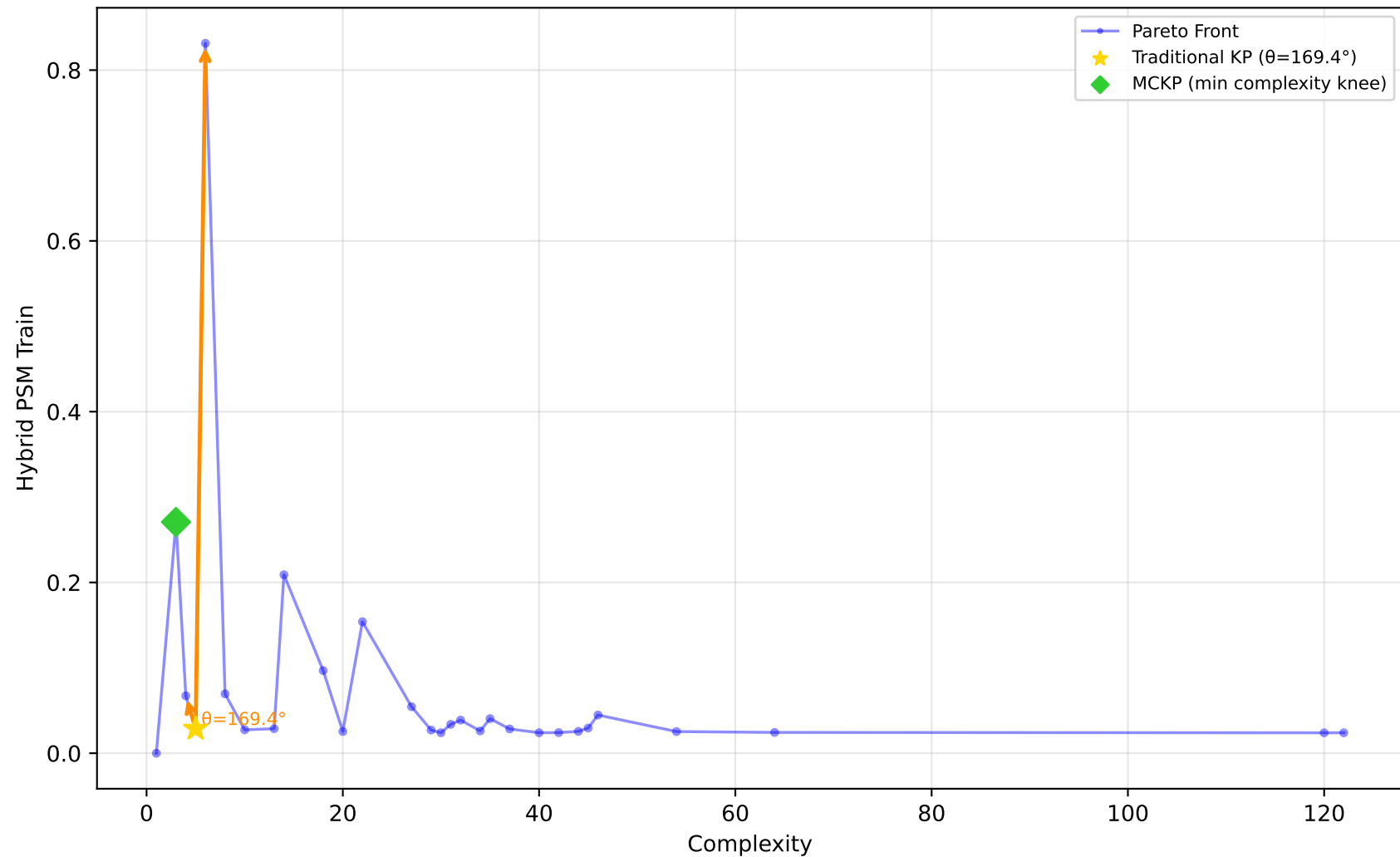
589_fri_c2_1000_25 - Run 3 - MVP - Hybrid PSM Train \lambda_1=0.30, \bar{\lambda}_2=0.00, \bar{\lambda}_3=0.20 | Difficulty: 1.00 | Method: hmr
