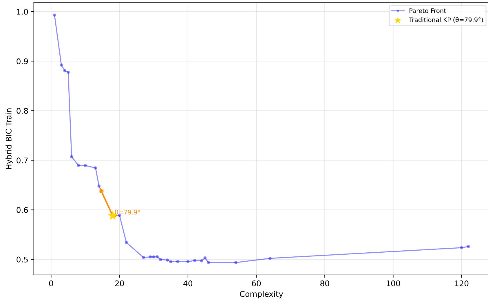
589_fri_c2_1000_25 - Run 3 - SVP - Hybrid BIC Train \lambda_1=0.10, \lambda_2=0.00, \lambda_3=0.10 | Difficulty: 1.00 | Method: hmr
