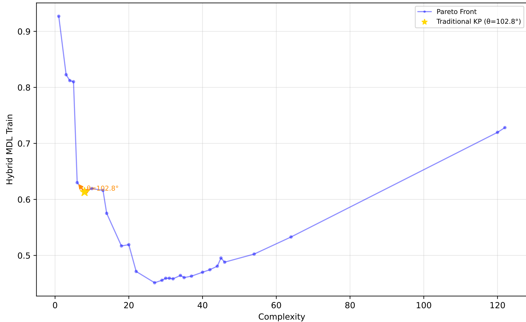
589_fri_c2_1000_25 - Run 3 - SVP - Hybrid MDL Train \lambda_1=0.10, \bar{\lambda}_2=0.00, \bar{\lambda}_3=0.10 | Difficulty: 1.00 | Method: hmr
