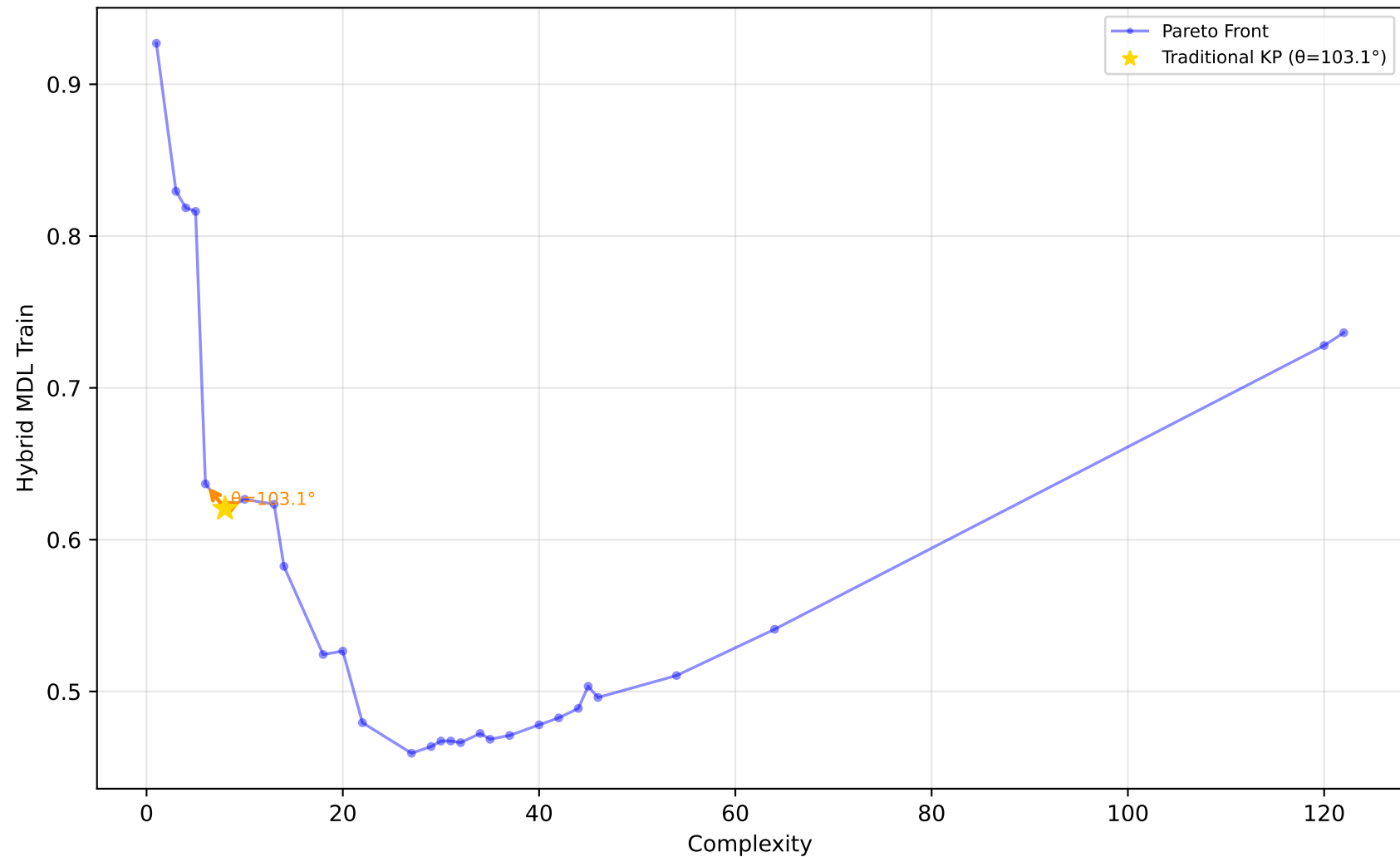
589_fri_c2_1000_25 - Run 3 - SVP - Hybrid MDL Train \lambda_1=0.20, \lambda_2=0.00, \lambda_3=1.00 | Difficulty: 1.00 | Method: hmr
