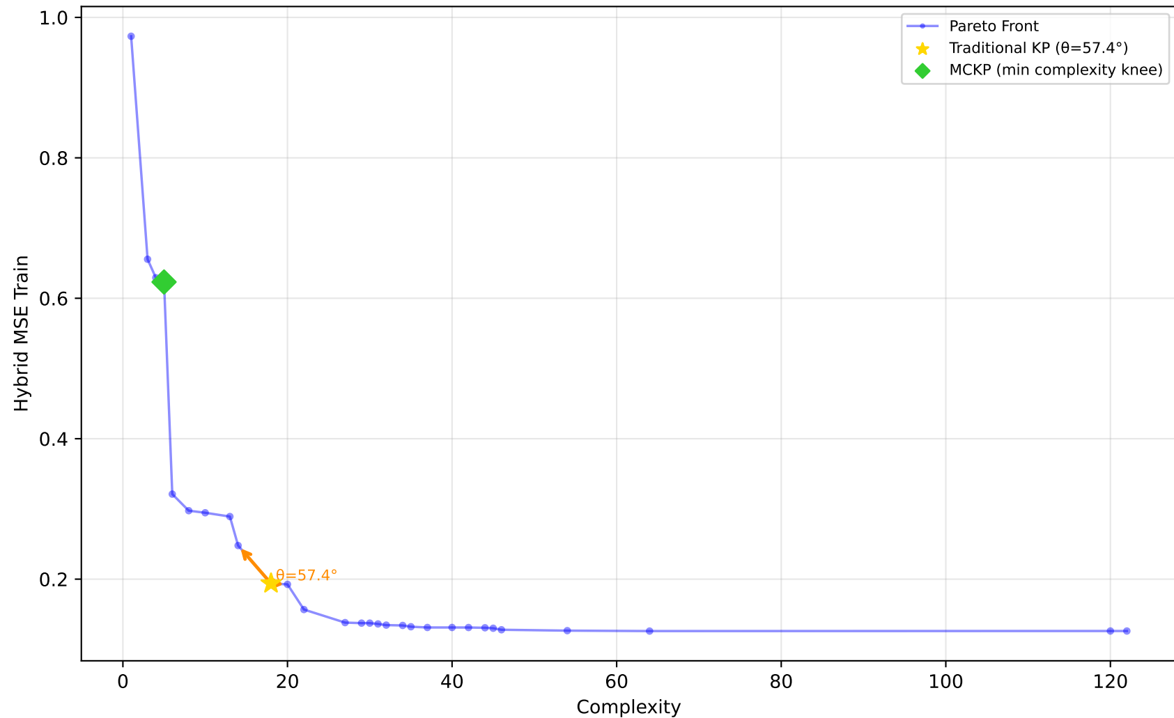
589_fri_c2_1000_25 - Run 3 - SVP - Hybrid MSE Train \lambda_1=0.20 , \lambda_2=0.00 , \lambda_3=1.00 | Difficulty: 1.00 | Method: hmr
