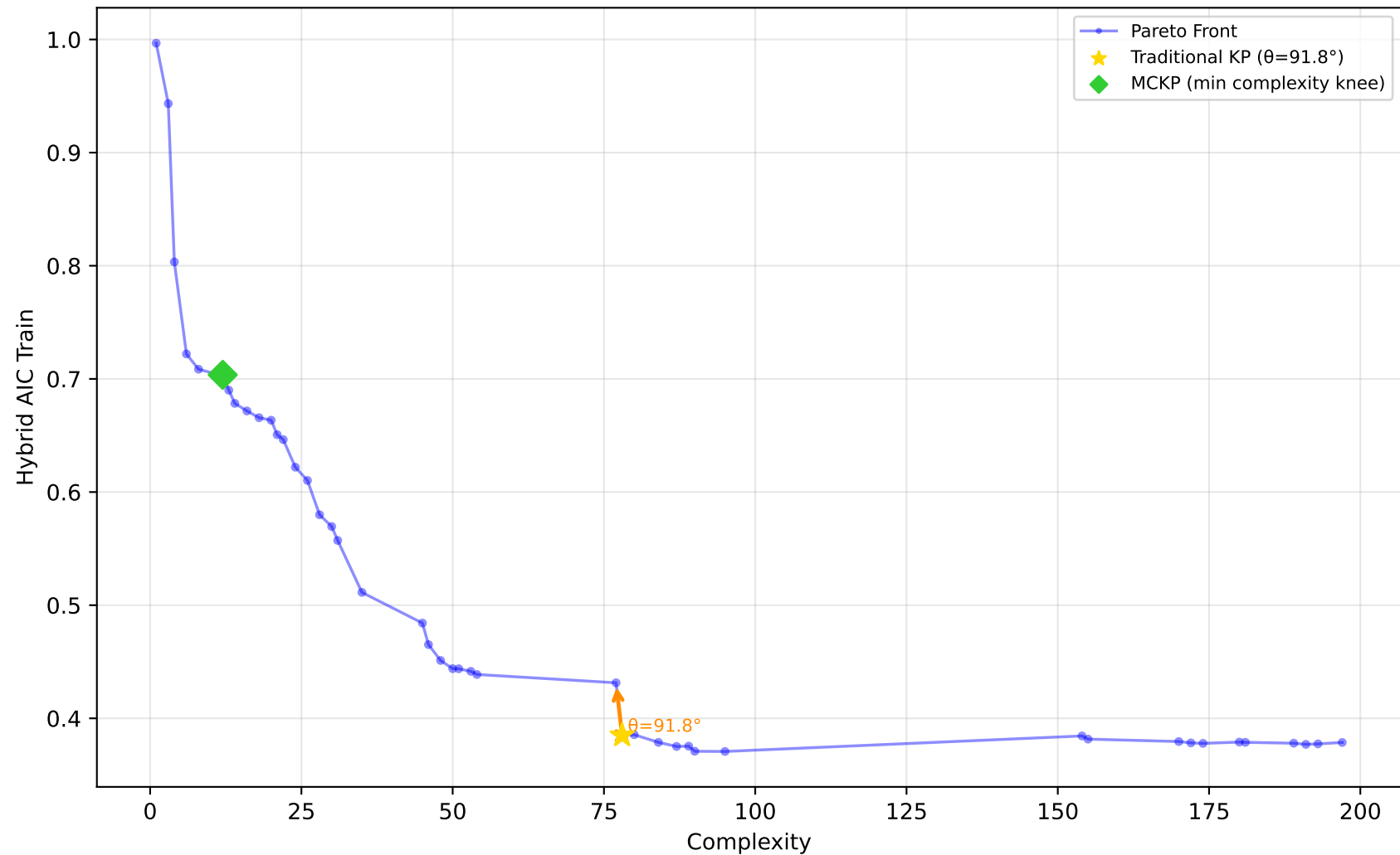
589_fri_c2_1000_25 - Run 4 - MVP - Hybrid AIC Train \lambda_1=0.00 , \lambda_2=0.00 , \lambda_3=0.00 | Difficulty: 1.00 | Method: hmr
