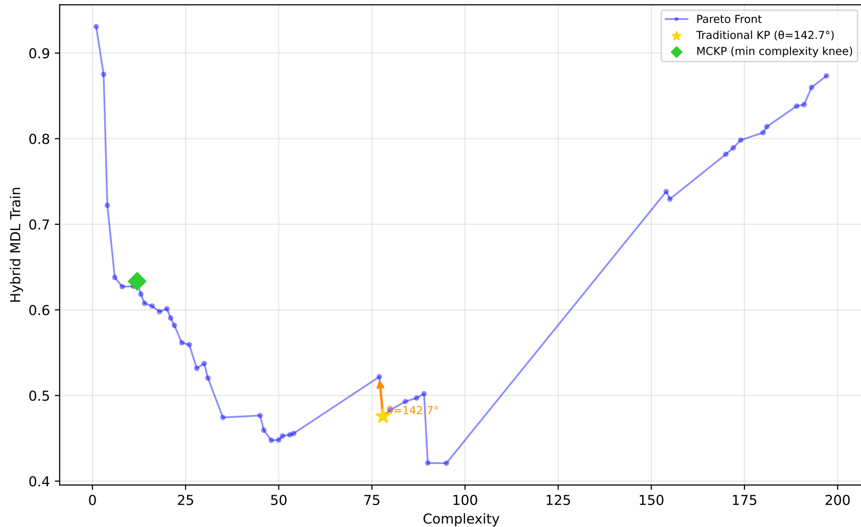
589_fri_c2_1000_25 - Run 4 - MVP - Hybrid MDL Train \lambda_1=0.00, \bar{\lambda}_2=0.00, \bar{\lambda}_3=0.00 | Difficulty: 1.00 | Method: hmr
