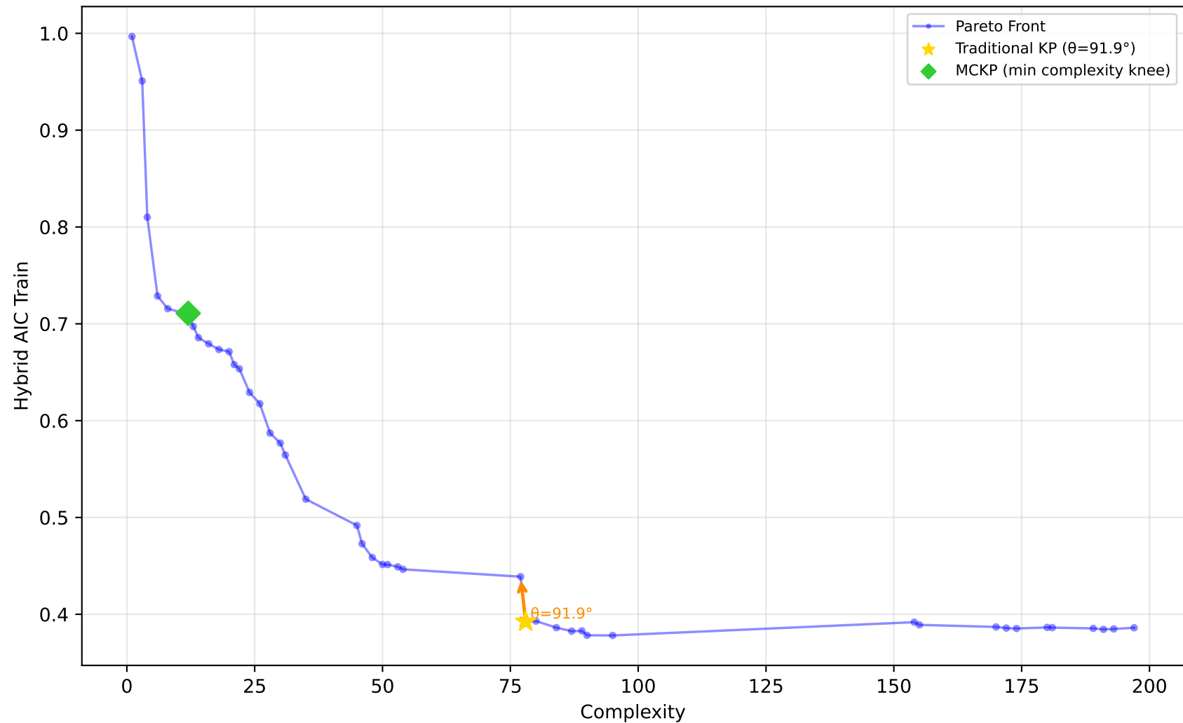
589_fri_c2_1000_25 - Run 4 - SVP - Hybrid AIC Train \lambda_1=0.10, \lambda_2=0.00, \lambda_3=0.10 | Difficulty: 1.00 | Method: hmr
