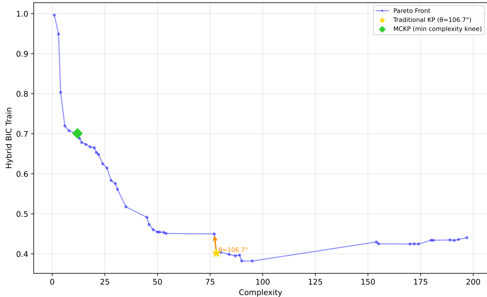
589_fri_c2_1000_25 - Run 4 - SVP - Hybrid BIC Train \lambda_1=0.10, \lambda_2=0.00, \lambda_3=0.10 | Difficulty: 1.00 | Method: hmr
