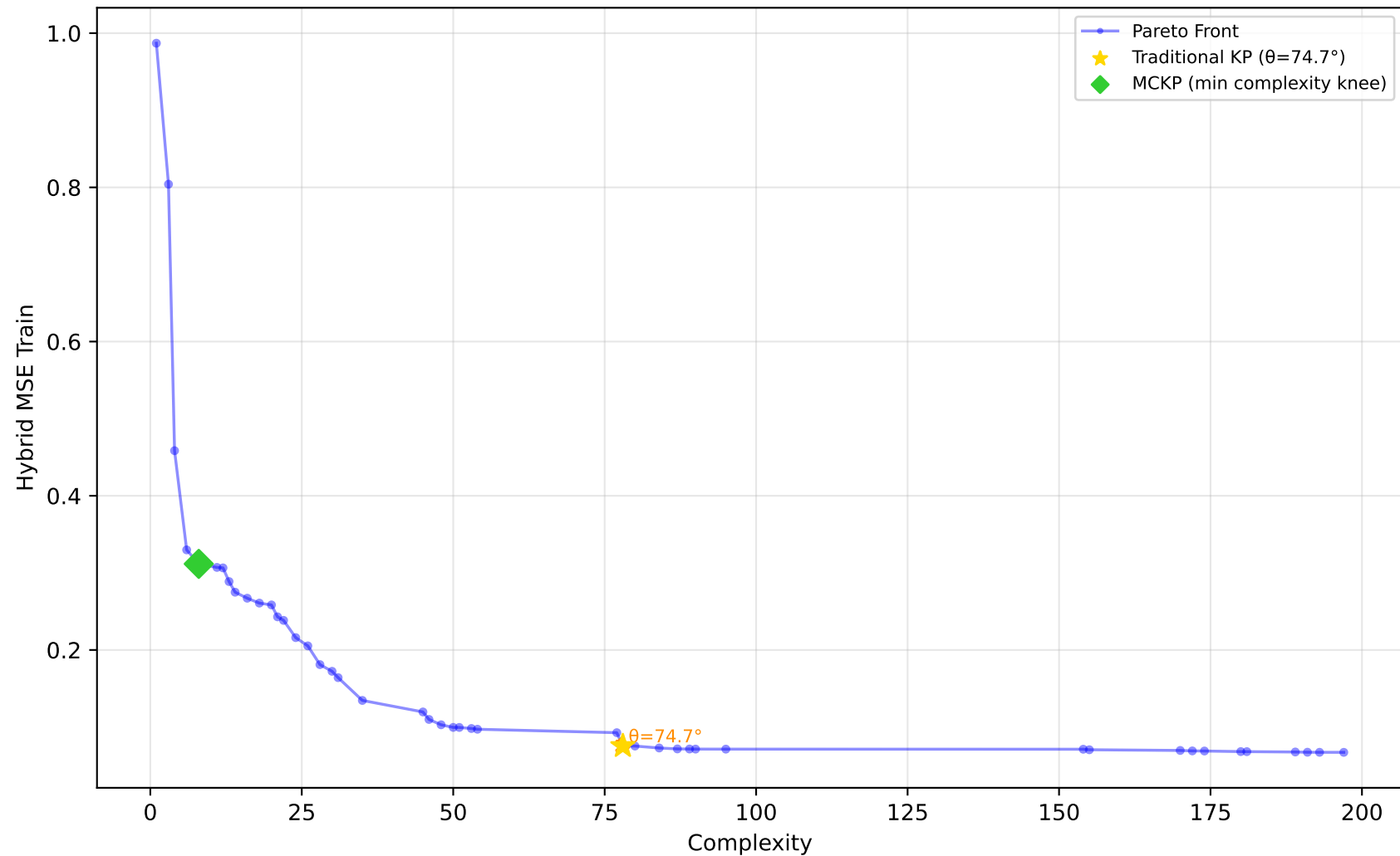
589_fri_c2_1000_25 - Run 4 - SVP - Hybrid MSE Train \lambda_1=0.10, \lambda_2=0.00, \lambda_3=0.10 | Difficulty: 1.00 | Method: hmr
