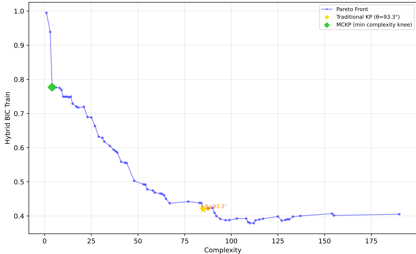
589_fri_c2_1000_25 - Run 5 - MVP - Hybrid BIC Train \lambda_1=0.00 , \lambda_2=0.00 , \lambda_3=0.00 | Difficulty: 1.00 | Method: hmr
