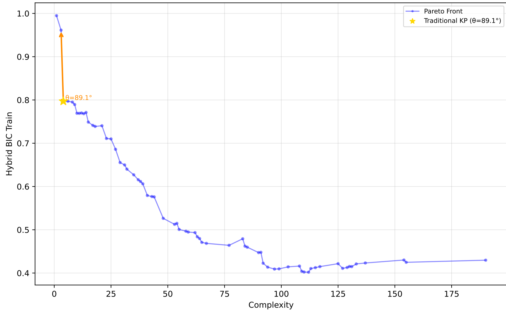
589_fri_c2_1000_25 - Run 5 - MVP - Hybrid BIC Train \lambda_1=0.30 , \lambda_2=0.00 , \lambda_3=0.20 | Difficulty: 1.00 | Method: hmr
