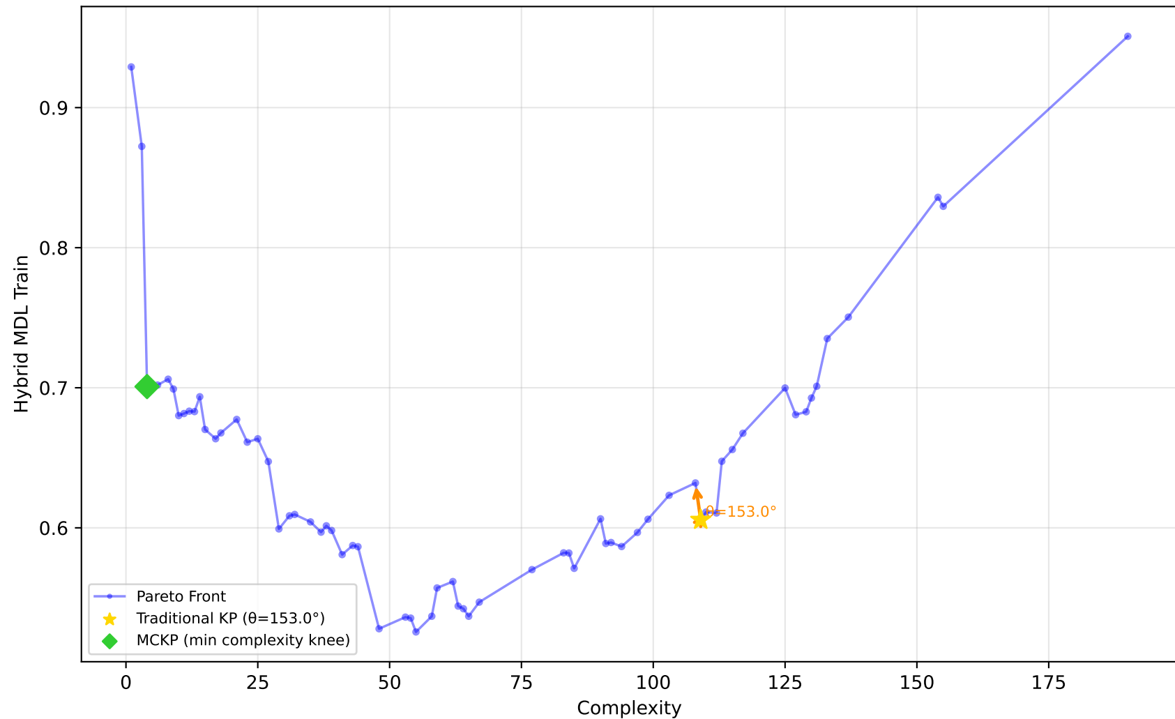
589_fri_c2_1000_25 - Run 5 - MVP - Hybrid MDL Train \lambda_1=0.00, \bar{\lambda}_2=0.00, \bar{\lambda}_3=0.00 | Difficulty: 1.00 | Method: hmr
