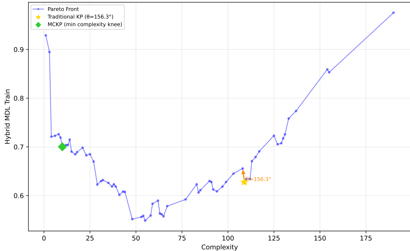
589_fri_c2_1000_25 - Run 5 - MVP - Hybrid MDL Train \lambda_1=0.30, \bar{\lambda}_2=0.00, \bar{\lambda}_3=0.20 | Difficulty: 1.00 | Method: hmr
