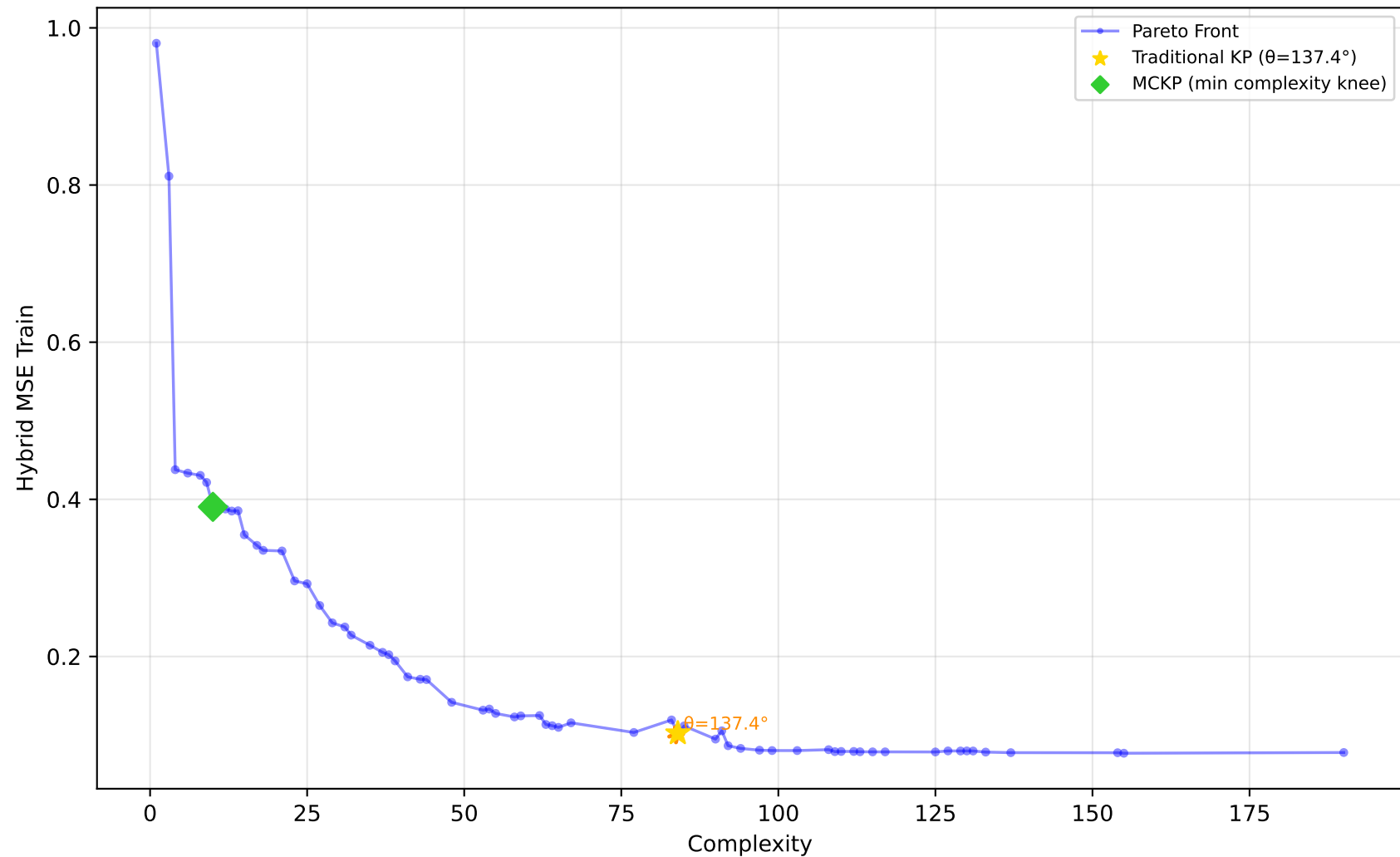
589_fri_c2_1000_25 - Run 5 - MVP - Hybrid MSE Train \lambda_1=0.30, \bar{\lambda}_2=0.00, \bar{\lambda}_3=0.20 | Difficulty: 1.00 | Method: hmr
