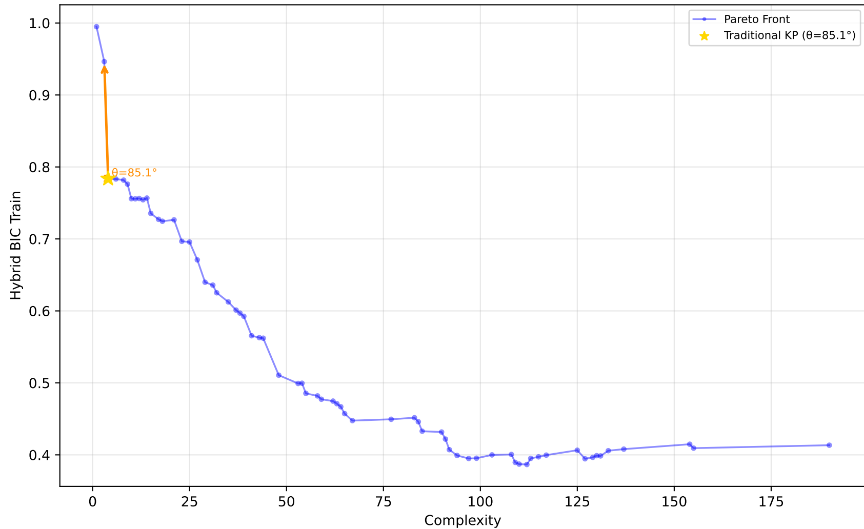
589_fri_c2_1000_25 - Run 5 - SVP - Hybrid BIC Train \lambda_1=0.10, \lambda_2=0.00, \lambda_3=0.10 | Difficulty: 1.00 | Method: hmr
