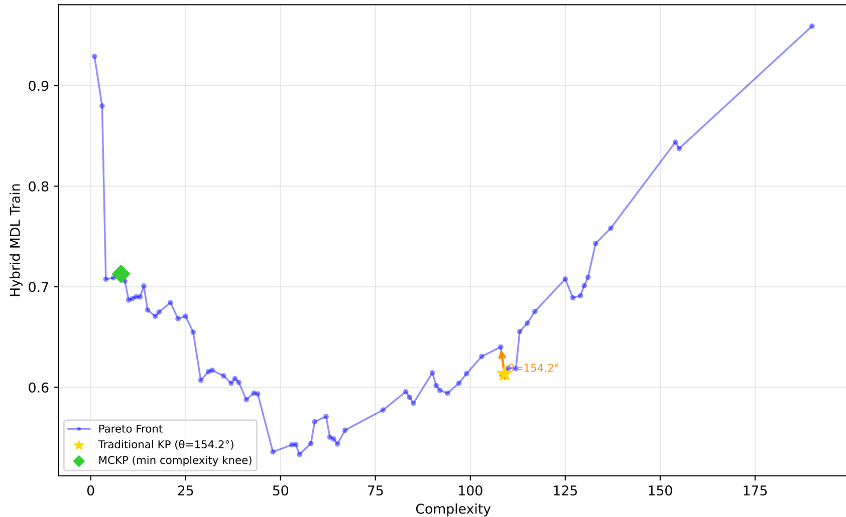
589_fri_c2_1000_25 - Run 5 - SVP - Hybrid MDL Train \lambda_1=0.10, \bar{\lambda}_2=0.00, \bar{\lambda}_3=0.10 | Difficulty: 1.00 | Method: hmr
