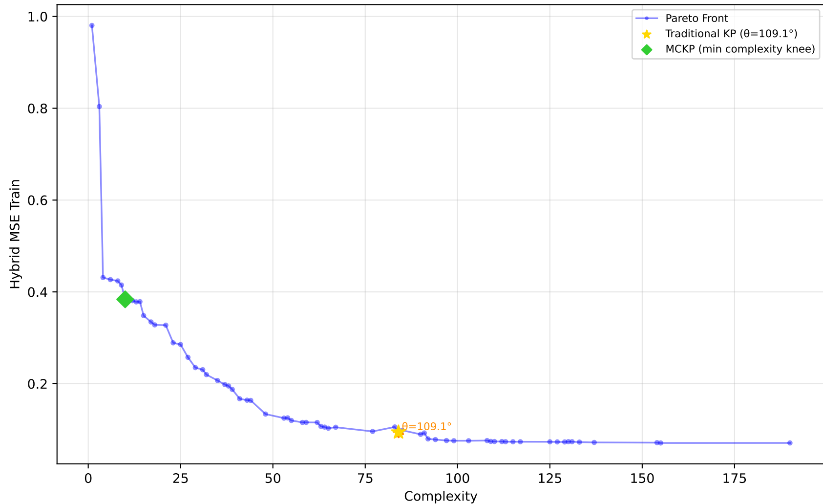
589_fri_c2_1000_25 - Run 5 - SVP - Hybrid MSE Train \lambda_1=0.20 , \lambda_2=0.00 , \lambda_3=1.00 | Difficulty: 1.00 | Method: hmr
