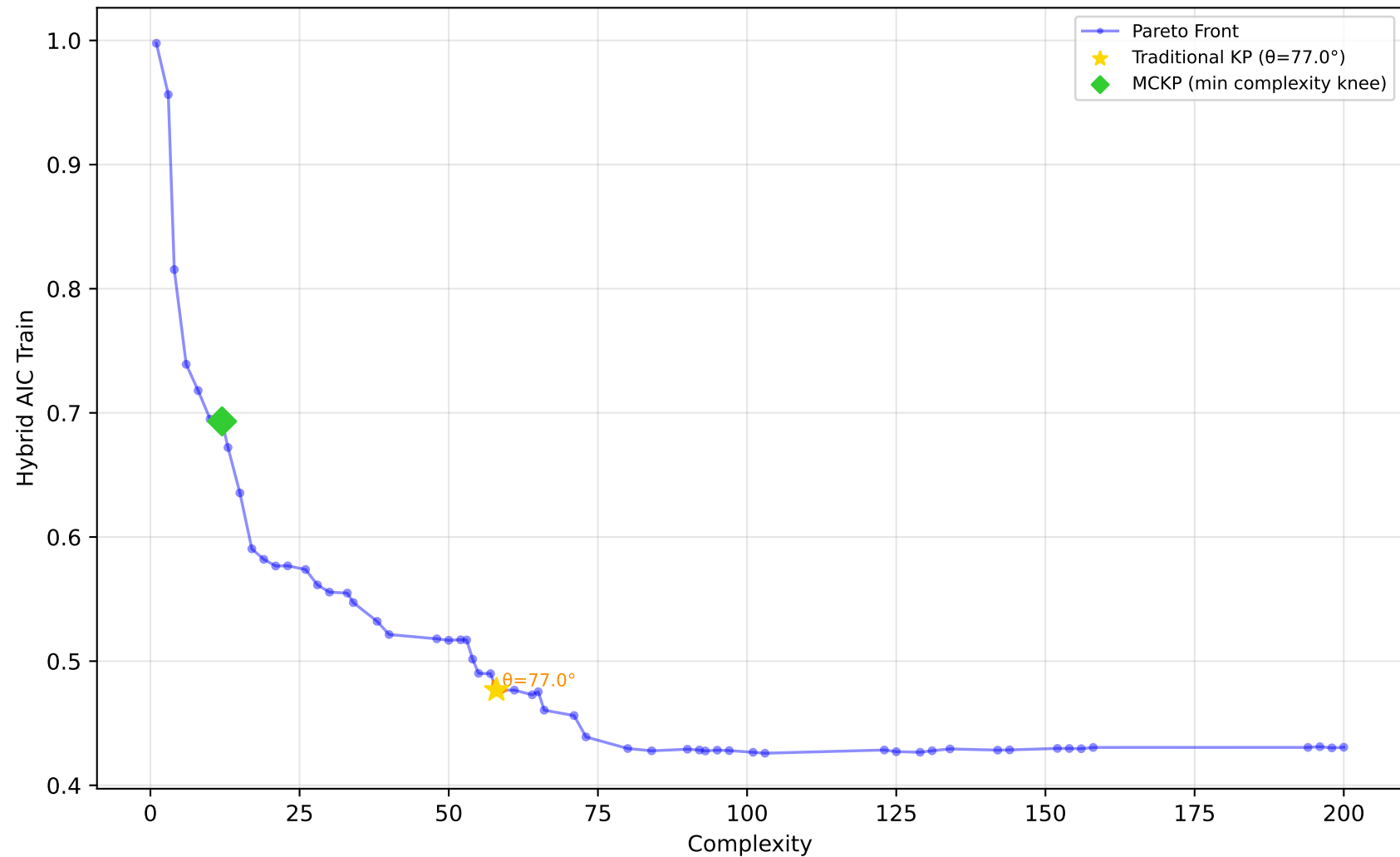
589_fri_c2_1000_25 - Run 6 - MVP - Hybrid AIC Train \lambda_1=0.00, \lambda_2=0.00, \lambda_3=0.00 | Difficulty: 1.00 | Method: hmr
