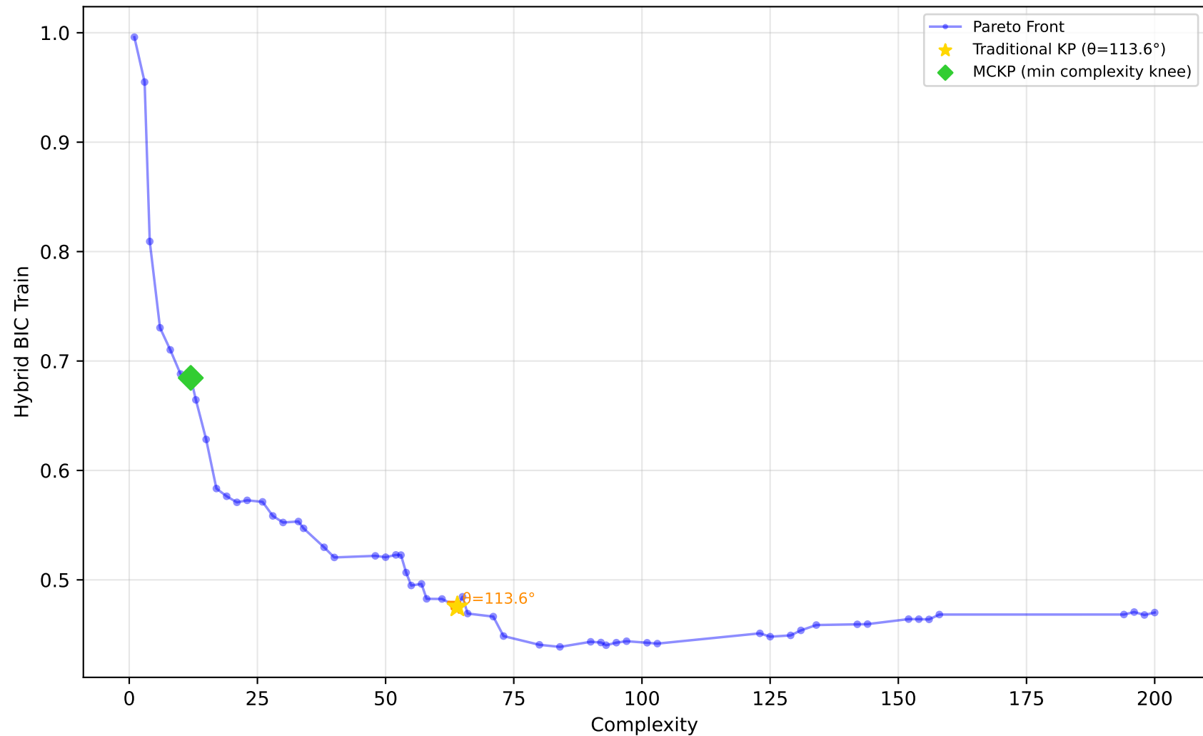
589_fri_c2_1000_25 - Run 6 - MVP - Hybrid BIC Train \lambda_1=0.00, \lambda_2=0.00, \lambda_3=0.00 | Difficulty: 1.00 | Method: hmr
