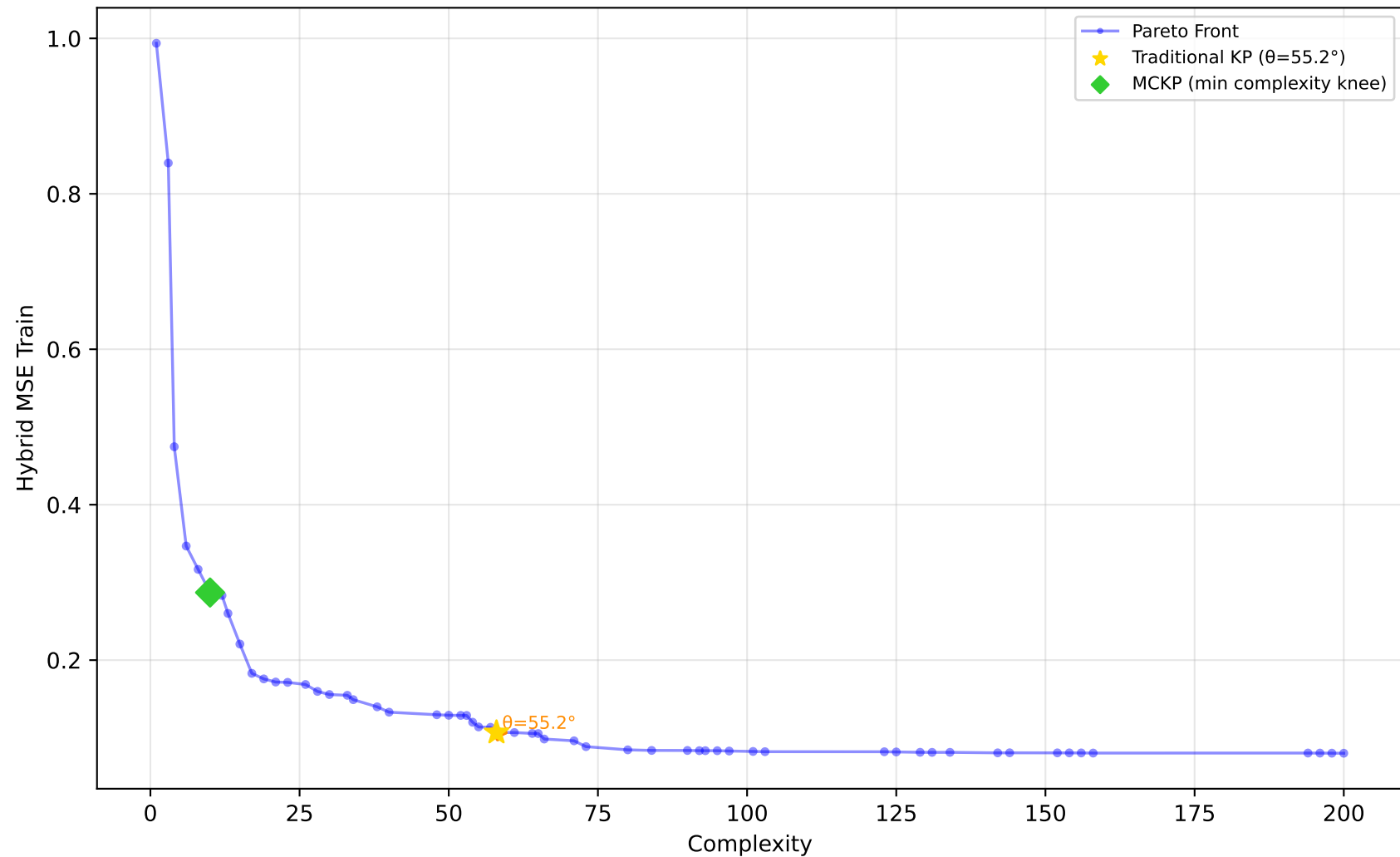
589_fri_c2_1000_25 - Run 6 - MVP - Hybrid MSE Train \lambda_1=0.00, \bar{\lambda}_2=0.00, \bar{\lambda}_3=0.00 | Difficulty: 1.00 | Method: hmr
