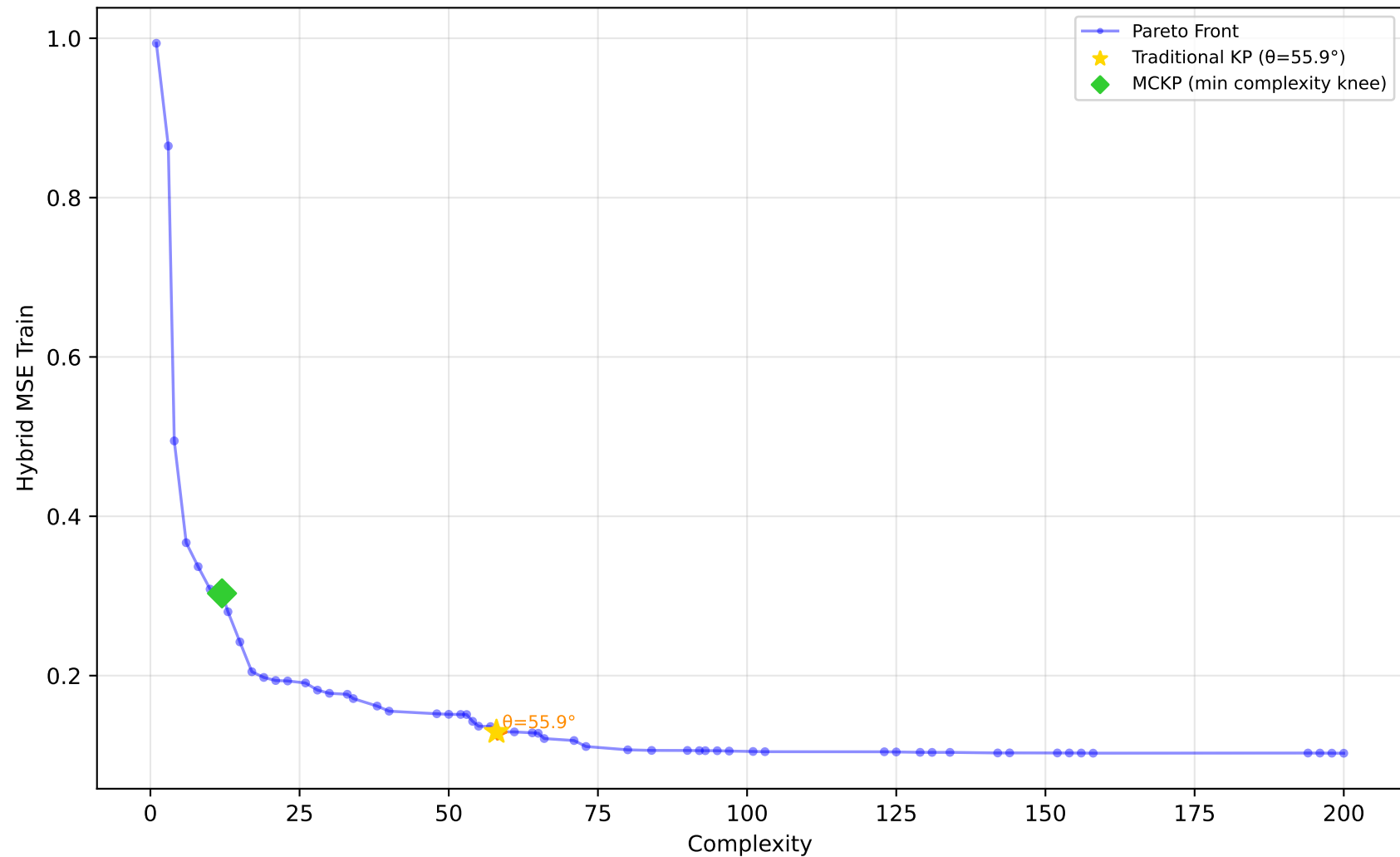
589_fri_c2_1000_25 - Run 6 - MVP - Hybrid MSE Train \lambda_1=0.30, \bar{\lambda}_2=0.00, \bar{\lambda}_3=0.20 | Difficulty: 1.00 | Method: hmr
