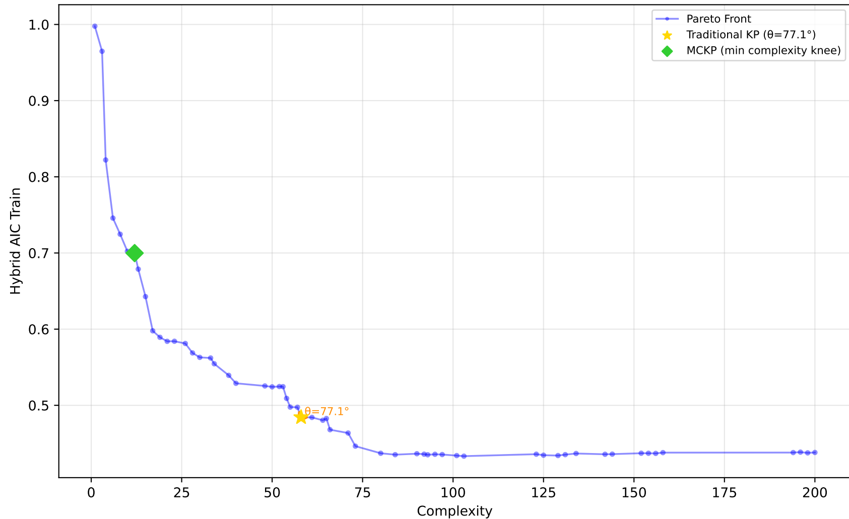
589_fri_c2_1000_25 - Run 6 - SVP - Hybrid AIC Train \lambda_1=0.10, \lambda_2=0.00, \lambda_3=0.10 | Difficulty: 1.00 | Method: hmr
