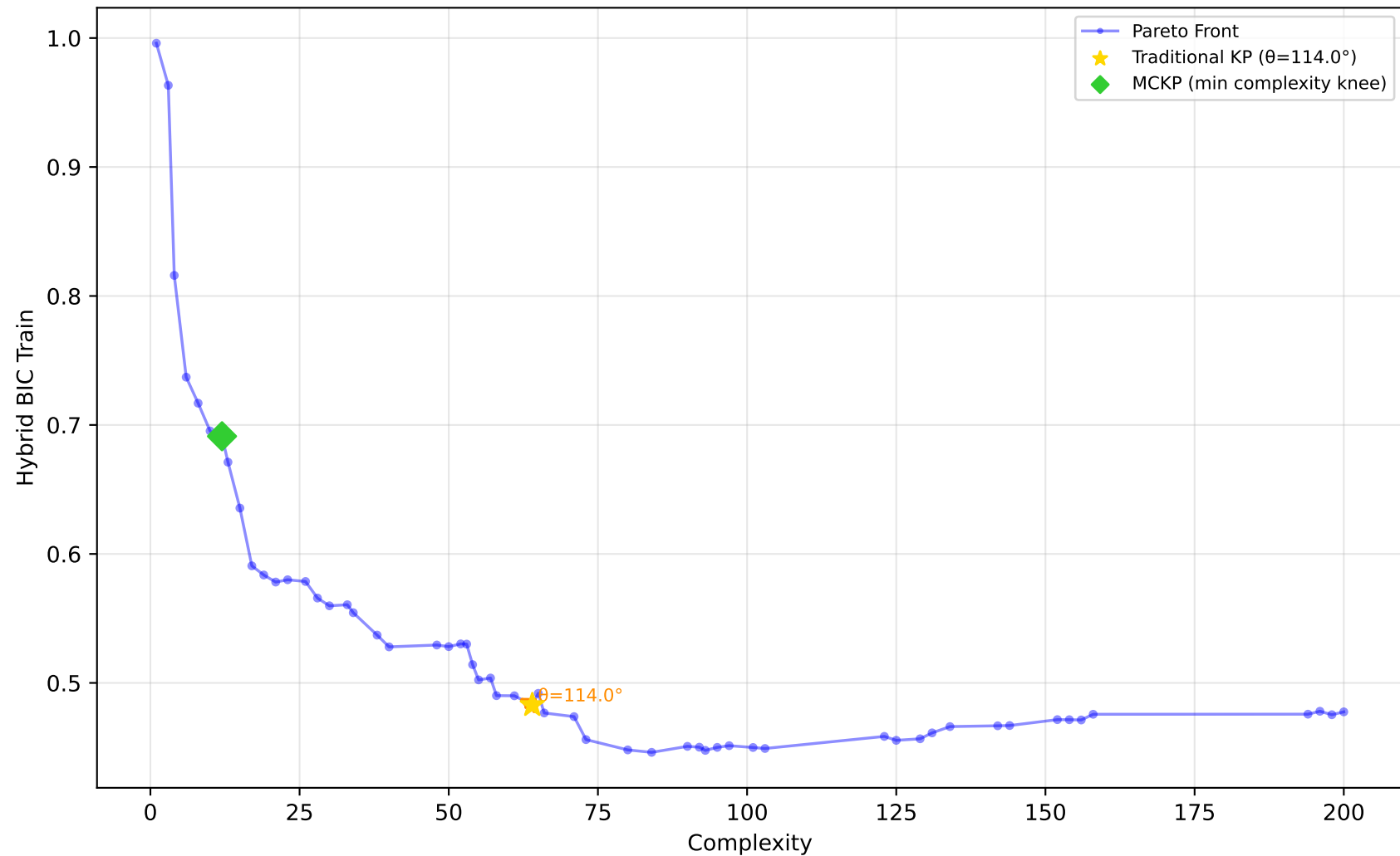
589_fri_c2_1000_25 - Run 6 - SVP - Hybrid BIC Train \lambda_1=0.10, \lambda_2=0.00, \lambda_3=0.10 | Difficulty: 1.00 | Method: hmr
