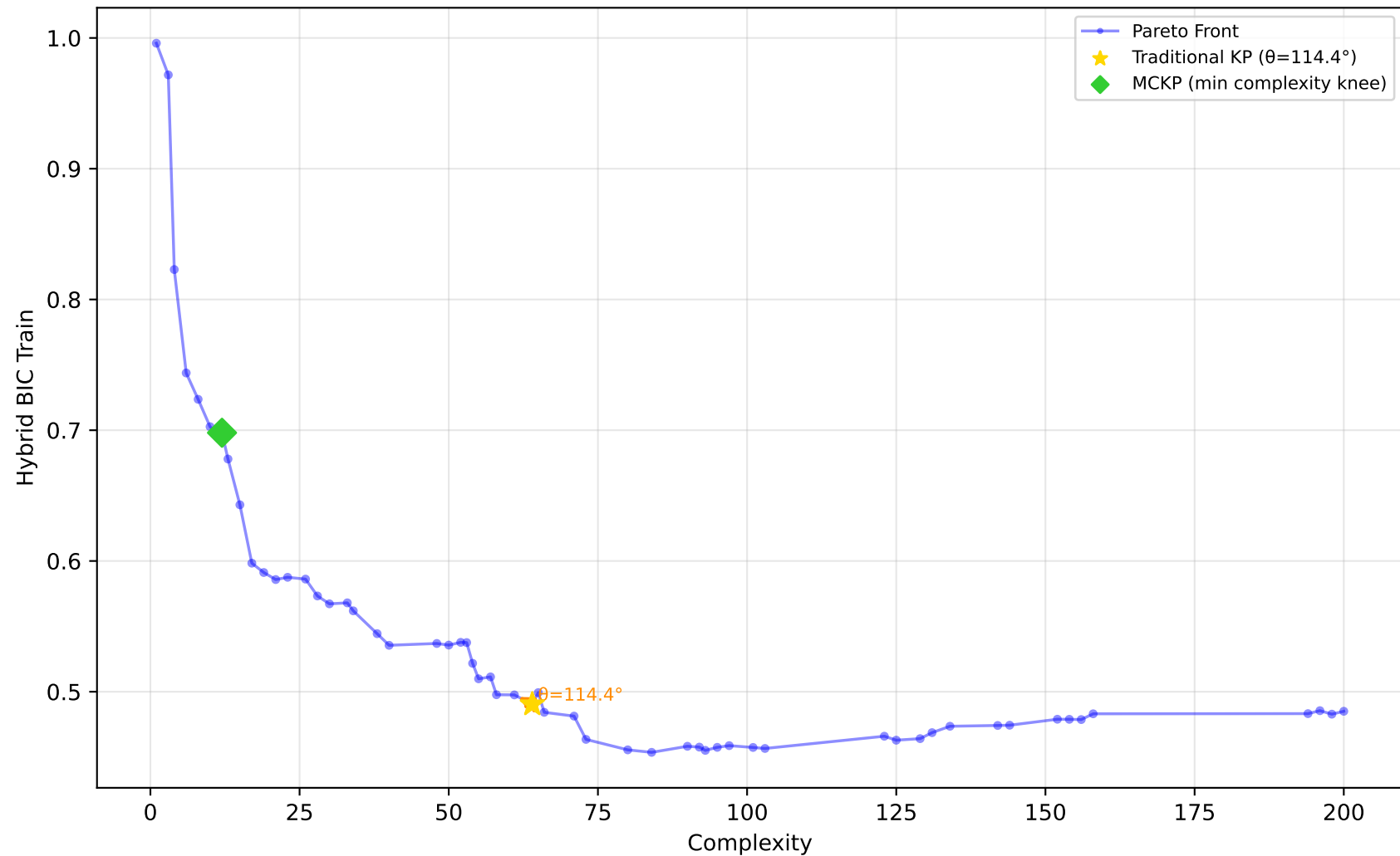
589_fri_c2_1000_25 - Run 6 - SVP - Hybrid BIC Train \lambda_1=0.20 , \lambda_2=0.00 , \lambda_3=1.00 | Difficulty: 1.00 | Method: hmr
